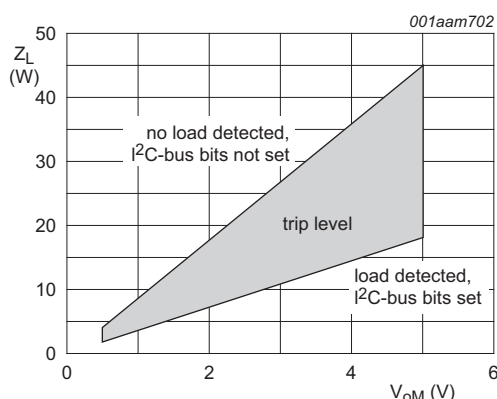
Fig 13. AC-load impedance as a function of peak output voltage (low current AC-load detection)
