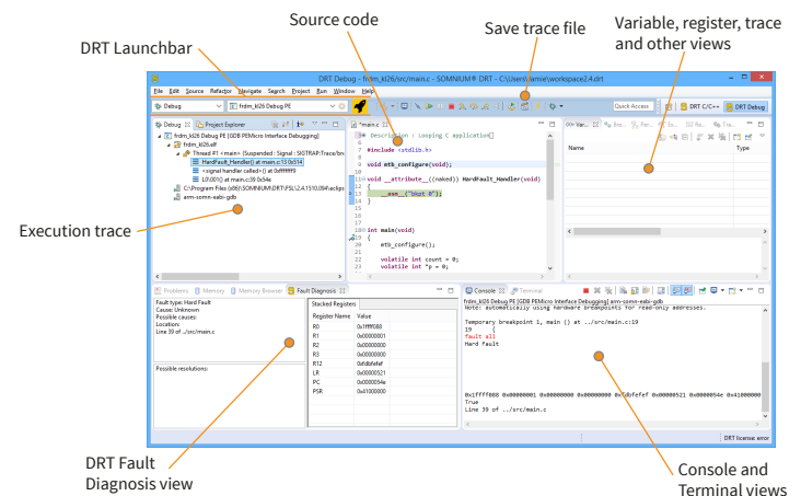
Figure 7: Multiple views available in DRT Debug
