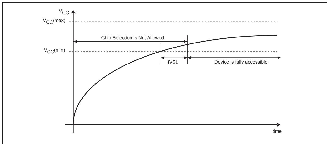
Figure 31. Power-up Timing
