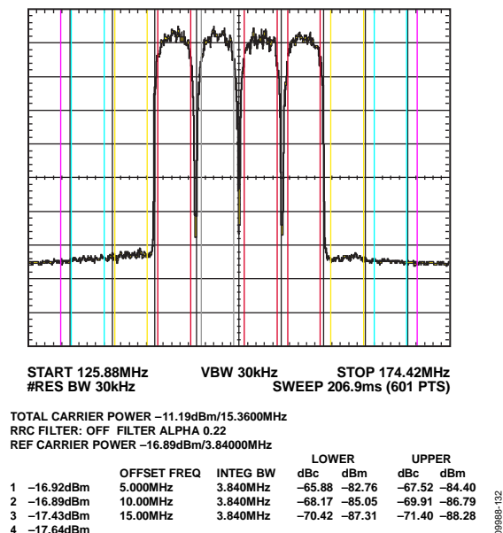
Figure 36. Four-Carrier W-CDMA ACLR Performance, IF = ~150 MHz
