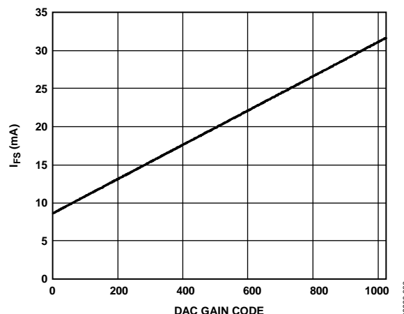
Figure 66. DAC Full-Scale Current vs. DAC Gain Code
