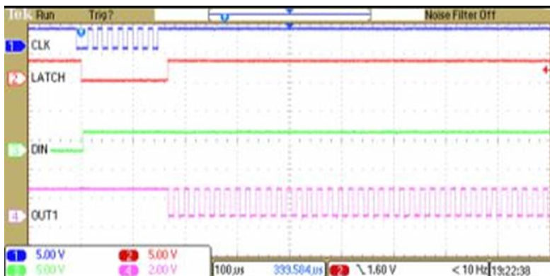
Figure 37. PWM Operation
