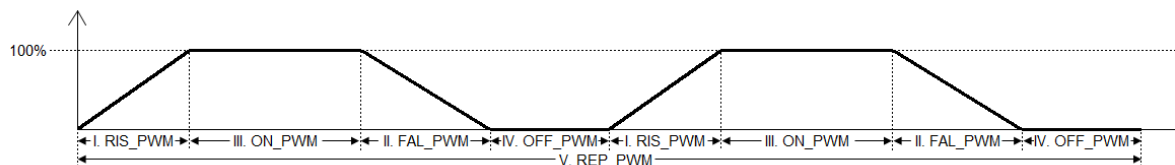
Figure 7. PWM waveform
