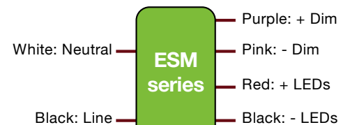
Wiring Diagram
