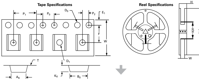
Dimensions for 0603, 0805, 1206, 1210, 1812 and 2920 size product (see table below)
