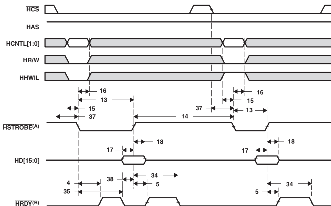
Figure 7-30 HPI16 Write Timing (HAS Not Used, Tied High)
