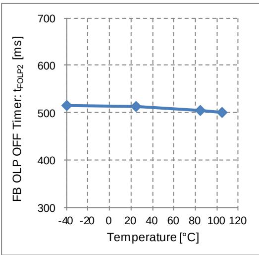
Figure 33. FB OLP OFF Timer vs Temperature
