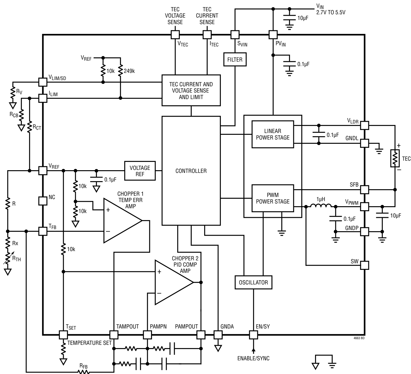
Figure 1. Simplified LTM4663 Block Diagram
