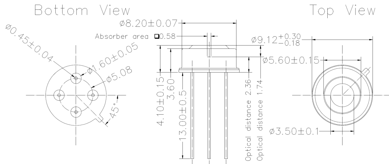
Figure 41 – Mechanical drawing of MLX90614xxA
