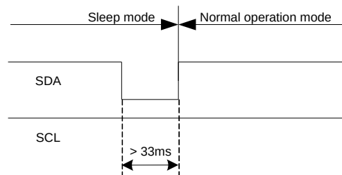
Figure 10 – Exit sleep mode (Wake Up Request)
