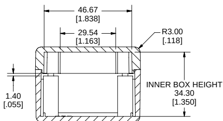
SECTION C-C SCALE 1 : 1
