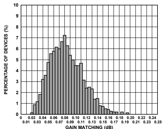
Figure 9. Channel-to-Channel Gain Matching (Gain = 34 dB)
