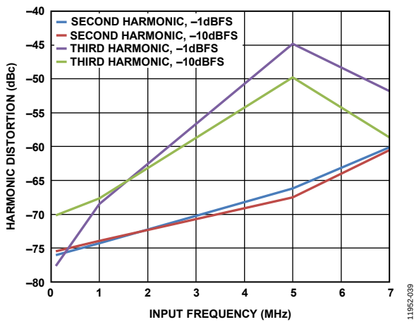
Figure 17. Harmonic Distortion vs. Input Frequency
