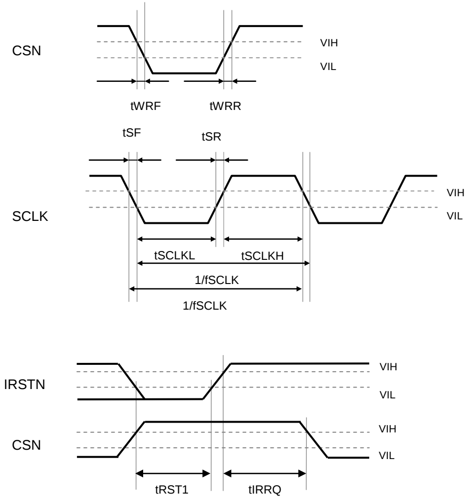
Figure 9. \mu\text{P} Interface 1 (SPI)
