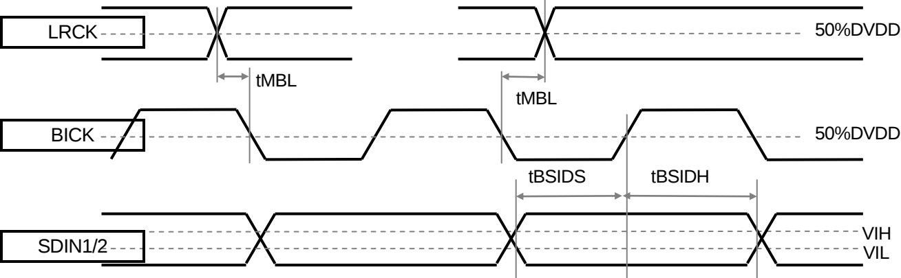
Figure 7. Audio Interface (Input Interface in Master Mode)
