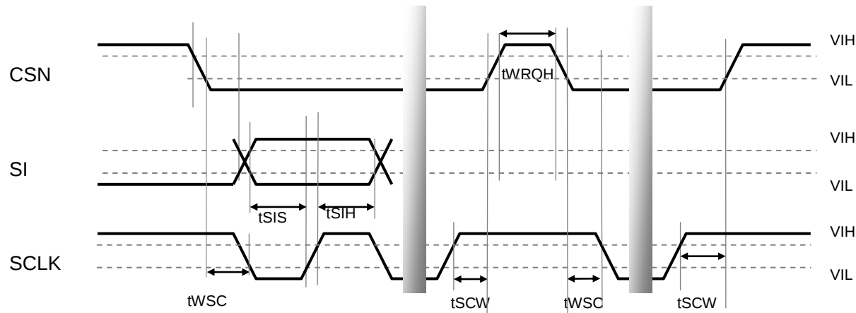
Figure 9. \mu\text{P} Interface 1 (SPI)
