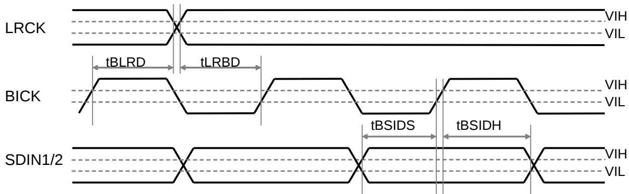
Figure 5. Audio Interface (Input Interface in Slave Mode)
