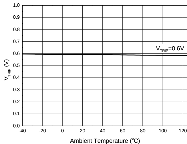
NTC Comparator Trip Threshold vs. Temperature
