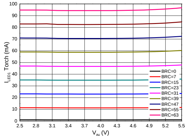
LED1 Torch Current vs. Input Voltage
