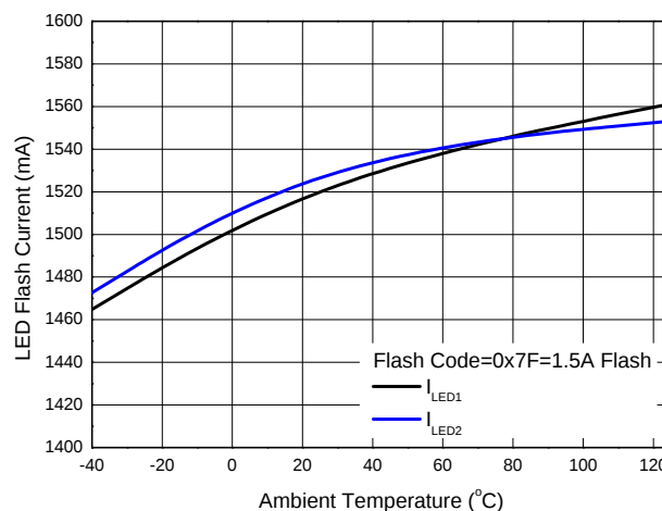
LED Flash Current vs. Temperature
