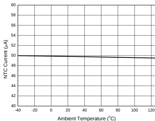
NTC Current vs. Temperature
