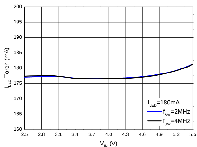
LED Torch Current vs. Input Voltage
