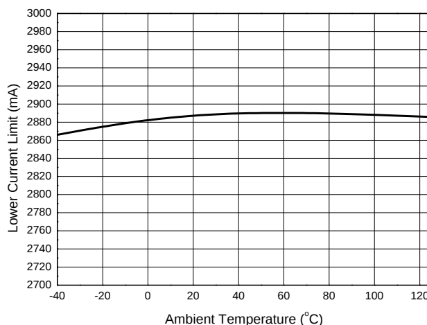
Inductor Current Limit 2 vs. Temperature
