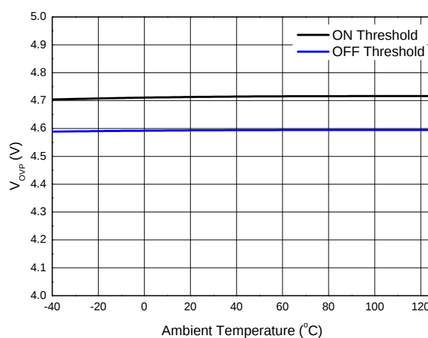
Over Voltage Protection Threshold vs. Temperature
