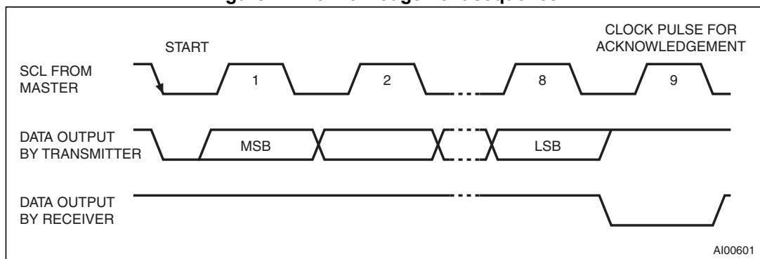
Figure 11. Acknowledgement sequence
