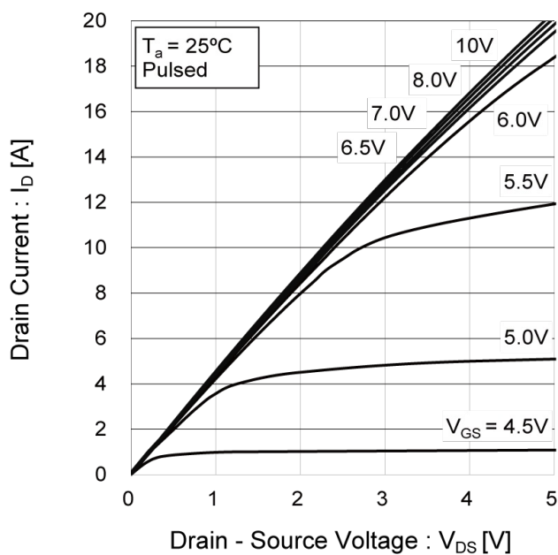
Fig.7 Output Characteristics(I)
