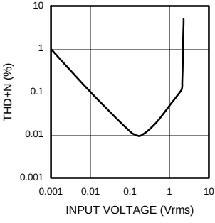
Fig.15 Total Harmonic Distortion ratio - Input Voltage (BD3870FS)
