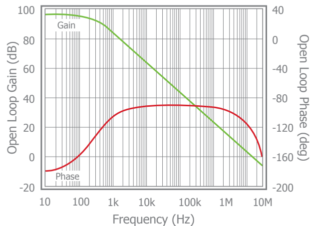
Open Loop Gain & Phase vs. Frequency
