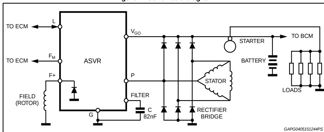
Figure 1: Schematic diagram
