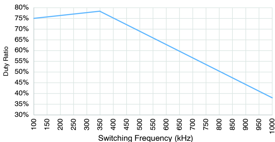
Figure 13. Maximum Duty Ratio vs. Switching Frequency
