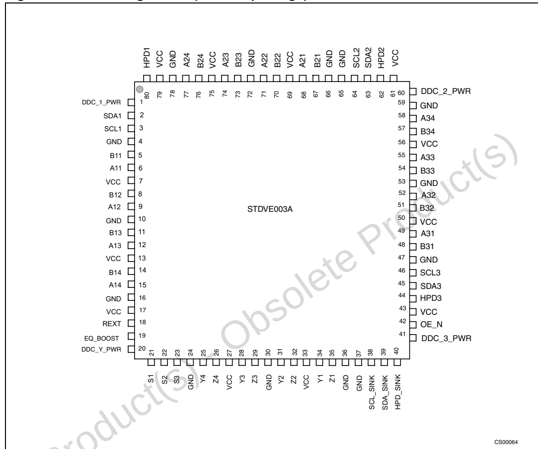
Figure 5. Pin configuration (TQFP80 package)
