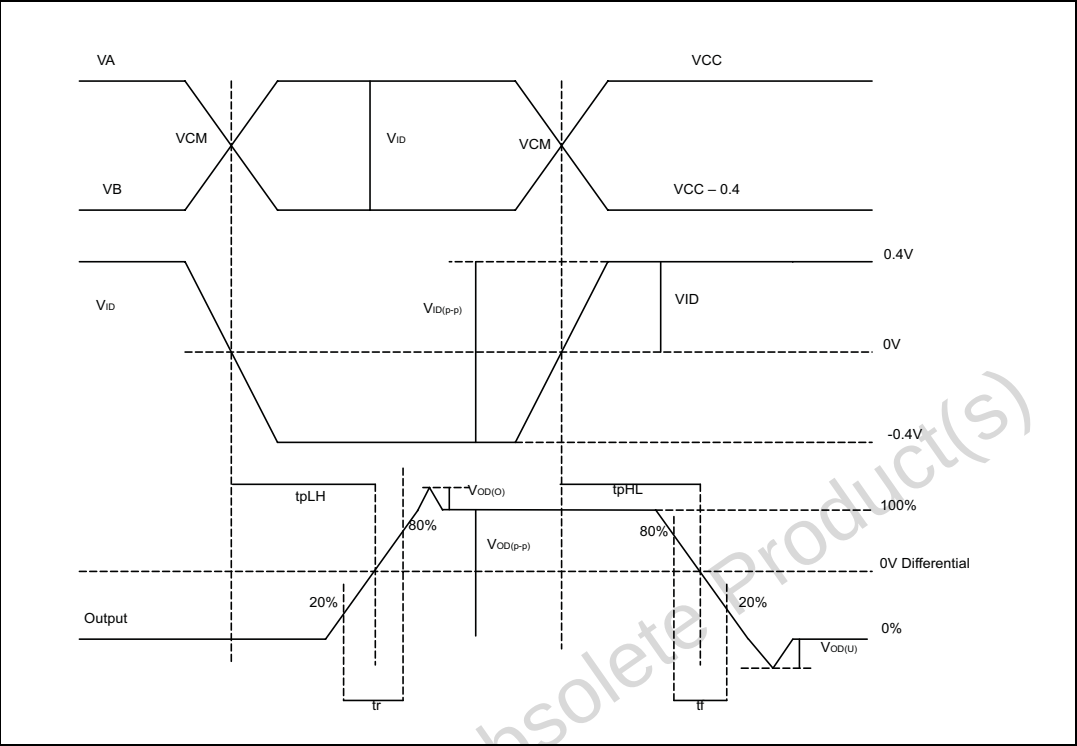
Figure 12. Propagation delays
