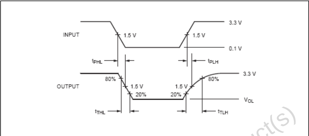
Figure 17. AC waveform 1 (I 2 C lines)
