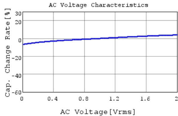
GRM31CR71C106KA12 C-AC Voltage capchange, D
