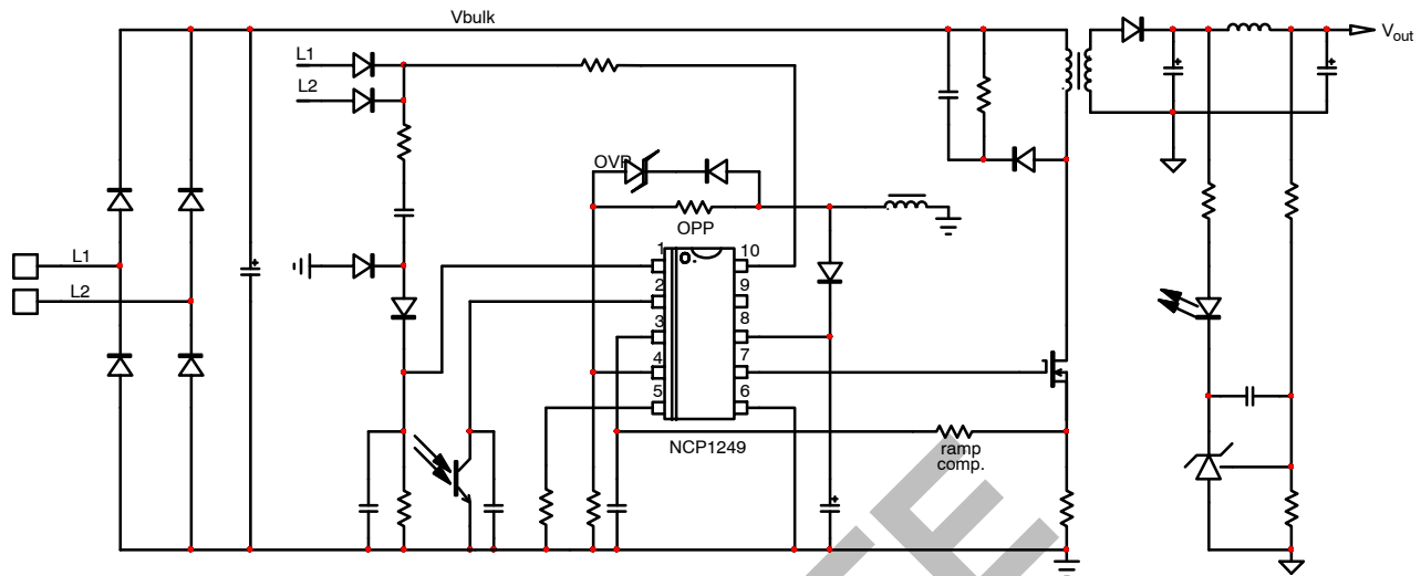
Figure 1. Typical Application Example
