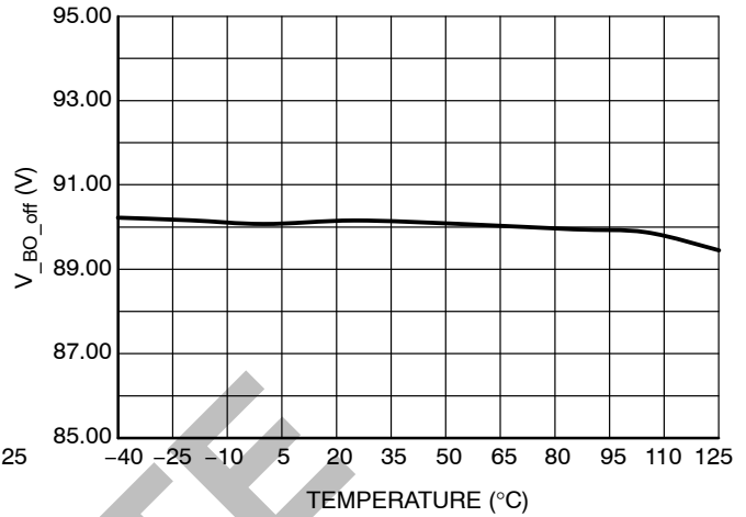
Figure 16. Brown-Out Turn-off Threshold, V BO_off
