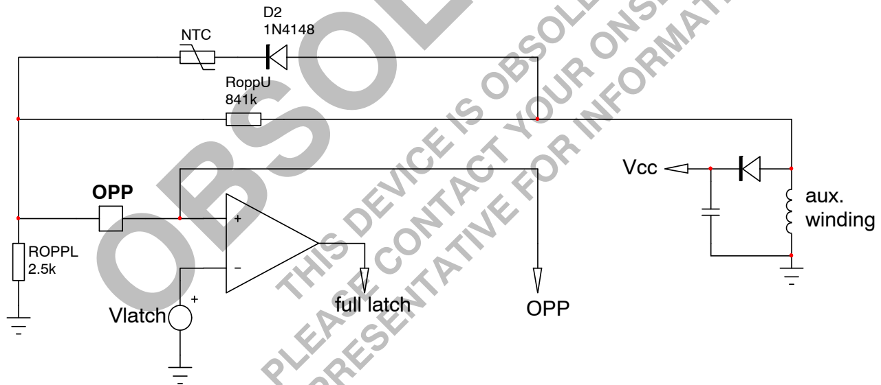
Figure 73. The Internal Circuitry Hooked to Pin 1 Can Be Used to Implement Over Temperature Protection (OTP)
