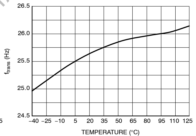
Figure 44. Transition Frequency Below Which Skip-cycle Occurs, f trans
