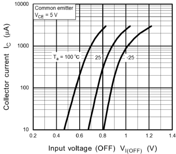
Fig. 11.4 RN1107MFV I_C - V_{I(OFF)}
