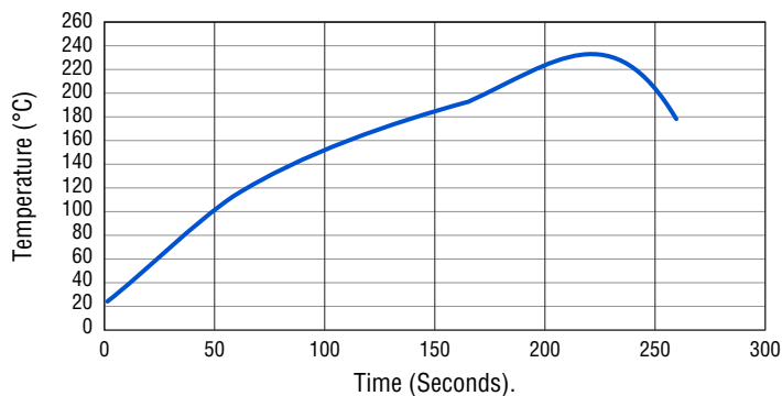
Recommended Reflow Profile
