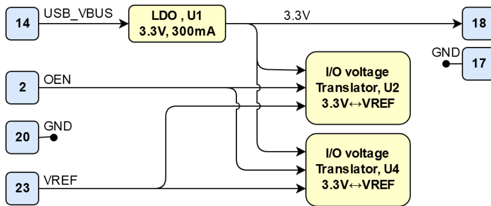
Figure 2: Power Distribution
