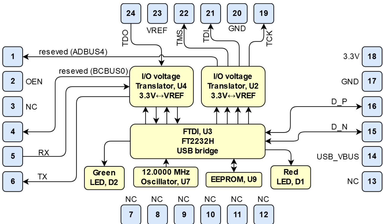
Figure 1: TEI0005 block diagram
