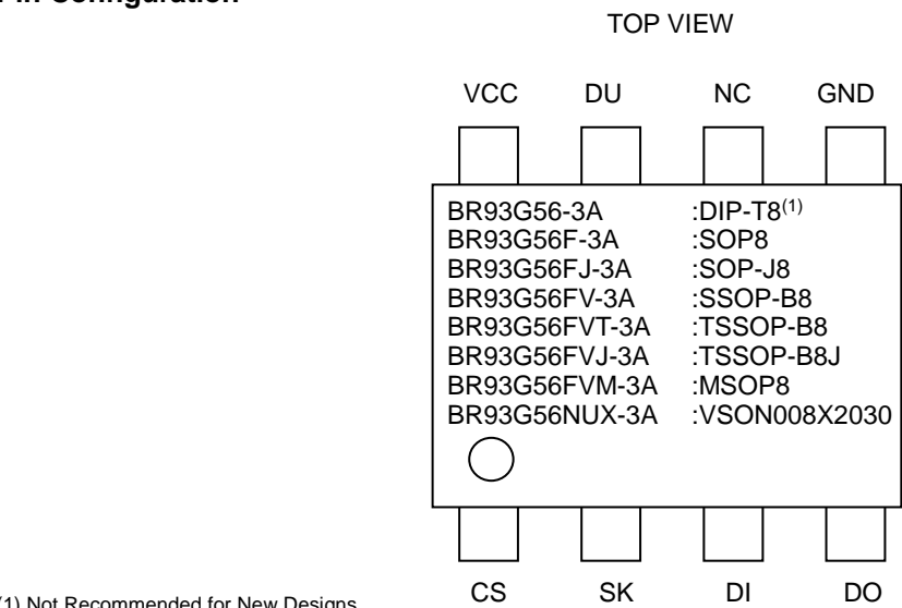
Figure 3. Pin Configuration
