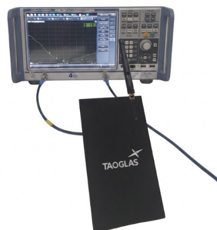
9x15cm Ground Plane
