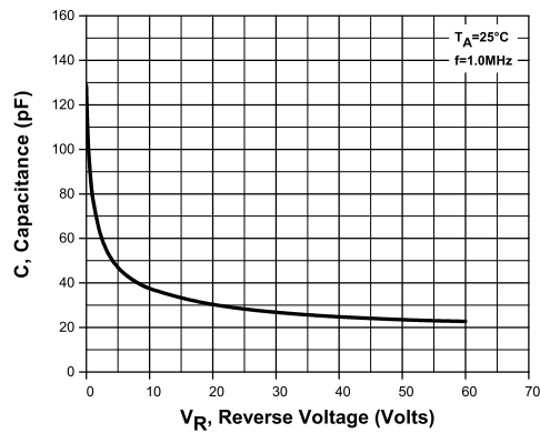
Capacitance for CMMSH1-60
