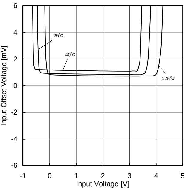
Figure 42. Input Offset Voltage - Input Voltage (VCC=5V)
