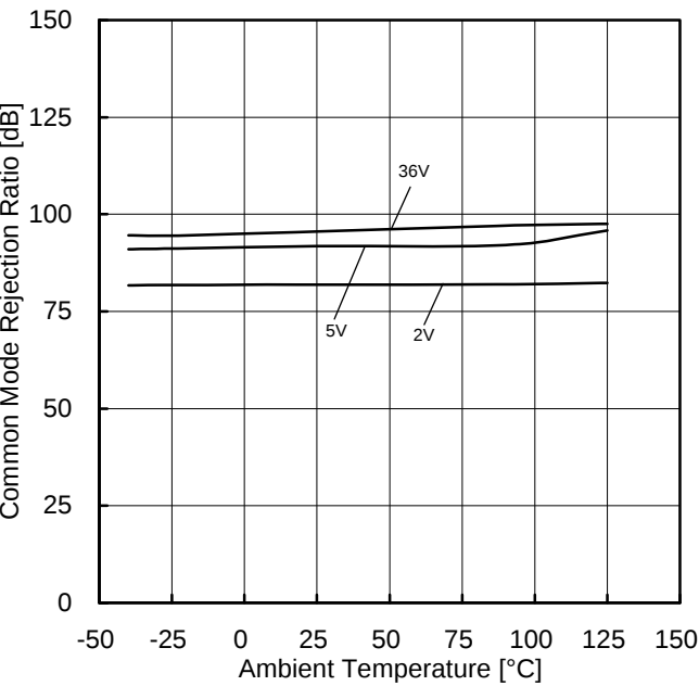
Figure 41. Common Mode Rejection Ratio vs Ambient Temperature
