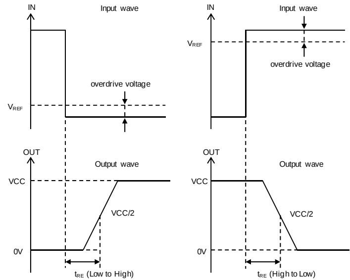
Figure 51. Response Time
