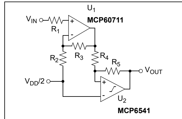
FIGURE 4-11: Precision Comparator.
