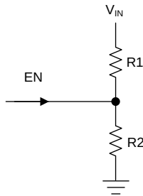
Figure 47. Undervoltage Lockout
