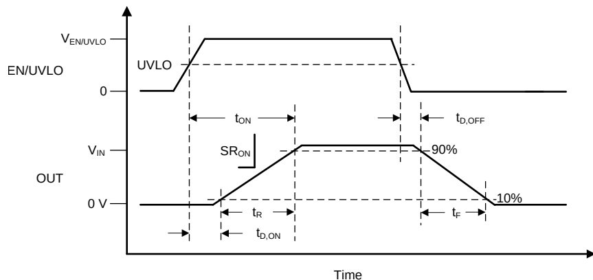
Figure 1. TPS2595x0, TPS2595x1, TPS2595x5 Switching Times
