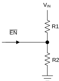
Figure 48. Overvoltage Lockout
