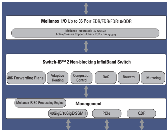
Figure 1. Mellanox Switch-IB 2 Architecture
