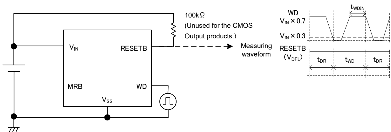
Circuit 7
