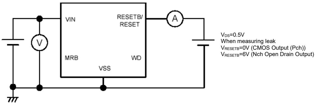
Circuit 4
