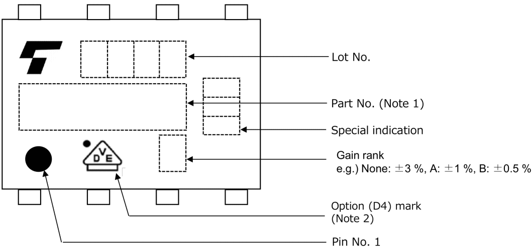
Fig. 16.3 Marking Example
