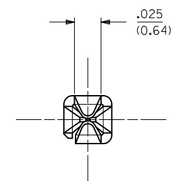
VIEW "B" - "B" SCALE = 16:1
