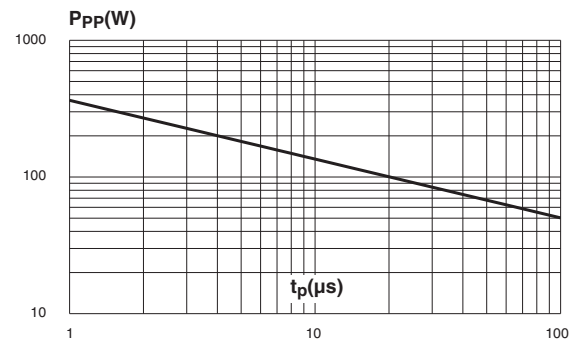
Figure 4: Peak power dissipation versus exponential pulse duration ( T_j initial = 25^{\circ}\text{C} )
