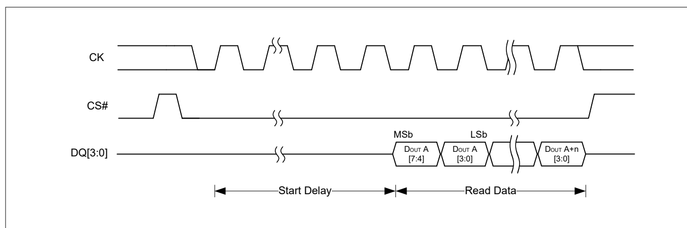
Figure 25 QPI transaction with output data sequence (AutoBoot)
