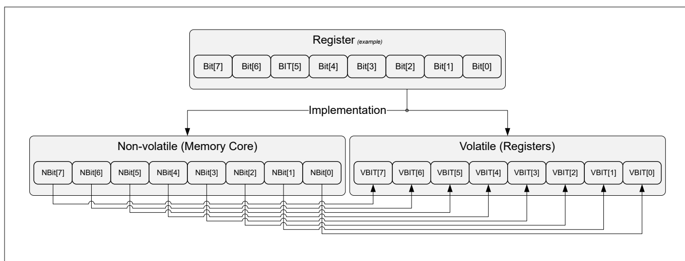
Figure 68 Register structure
