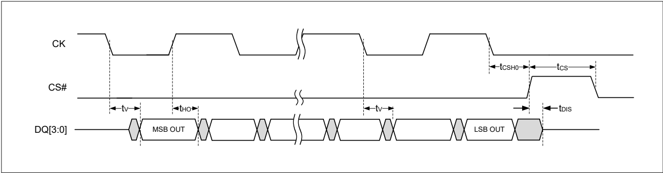
Figure 84 Quad and QPI DDR output timing
