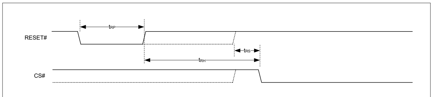
Figure 56 Hardware reset using RESET# input (reset pulse = t_{RP} (min))
