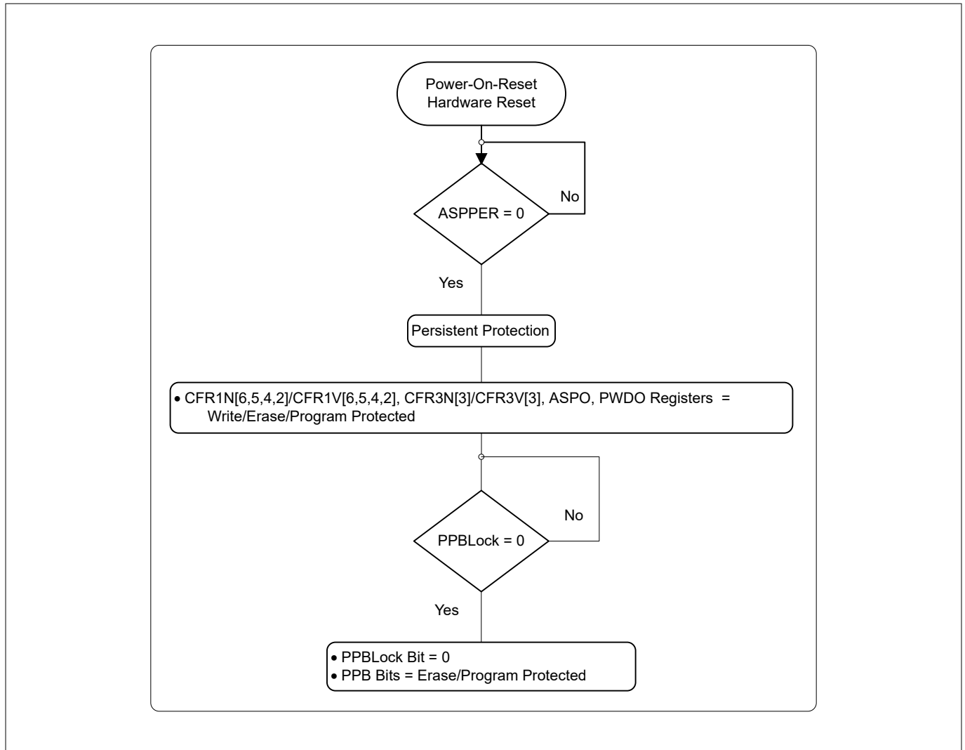
Figure 47 Persistent protection scheme flowchart
