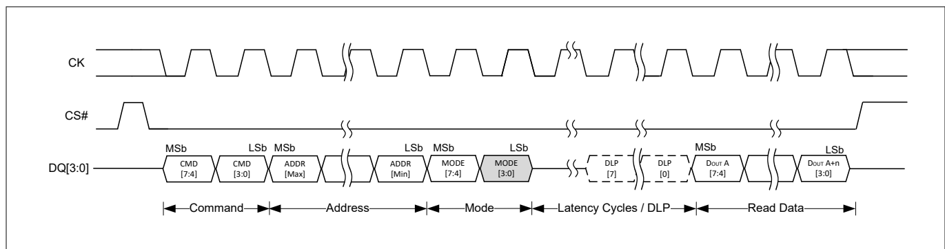
Figure 32 QPI SDR read transaction with command, address, and mode input (output latency) 6)
