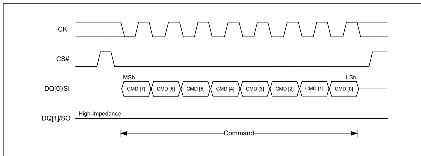
Figure 7 SPI transaction with command input
