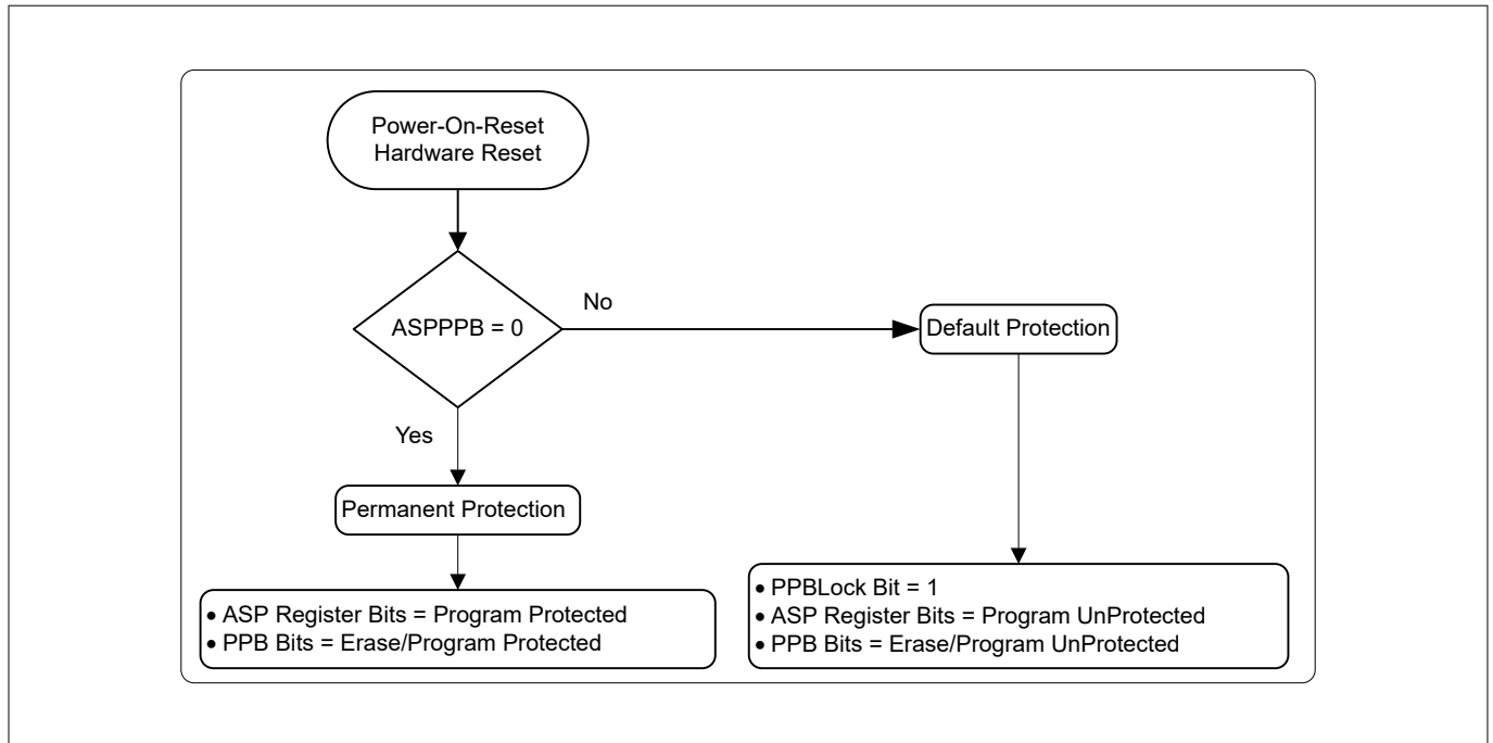
Figure 49 Permanent PPB sector protection flowchart
