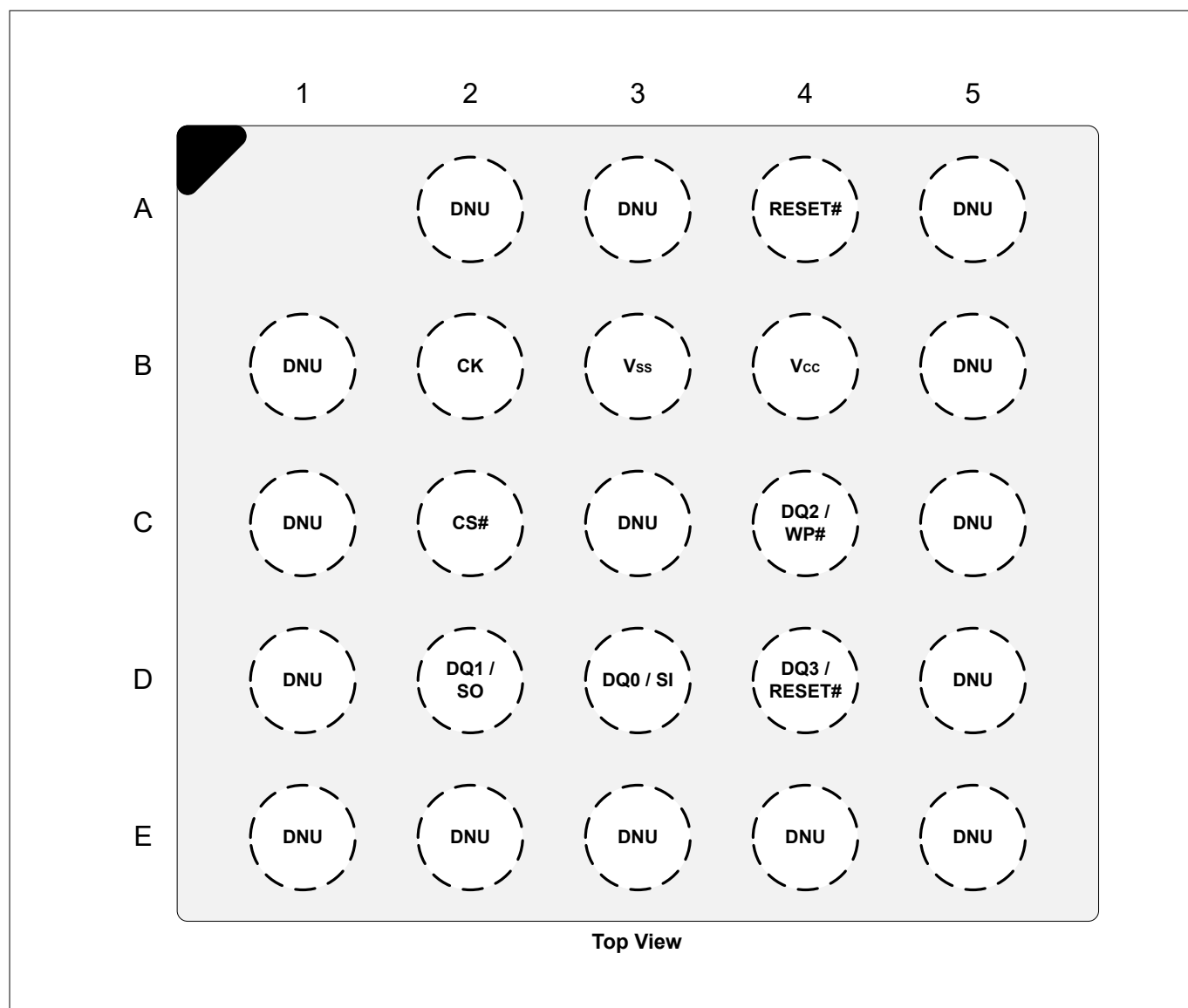
Figure 1 24-ball BGA pinout configuration 1)
