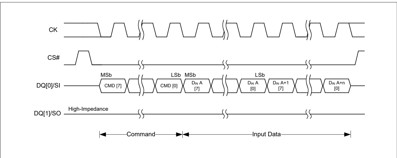
Figure 11 SPI program transaction with command and data input
