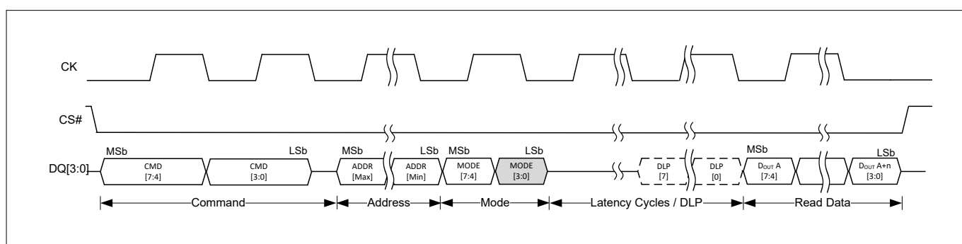
Figure 34 QPI DDR read transaction with command, address, and mode input (output latency) 6)
