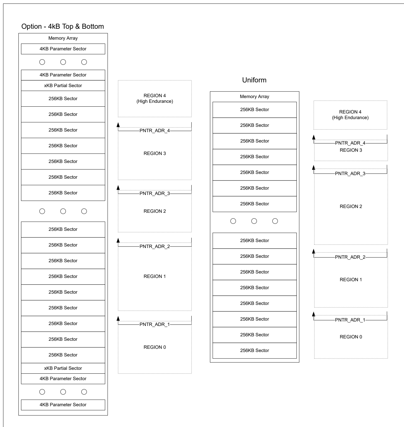
Figure 42 Infineon Endurance Flex architecture overview
