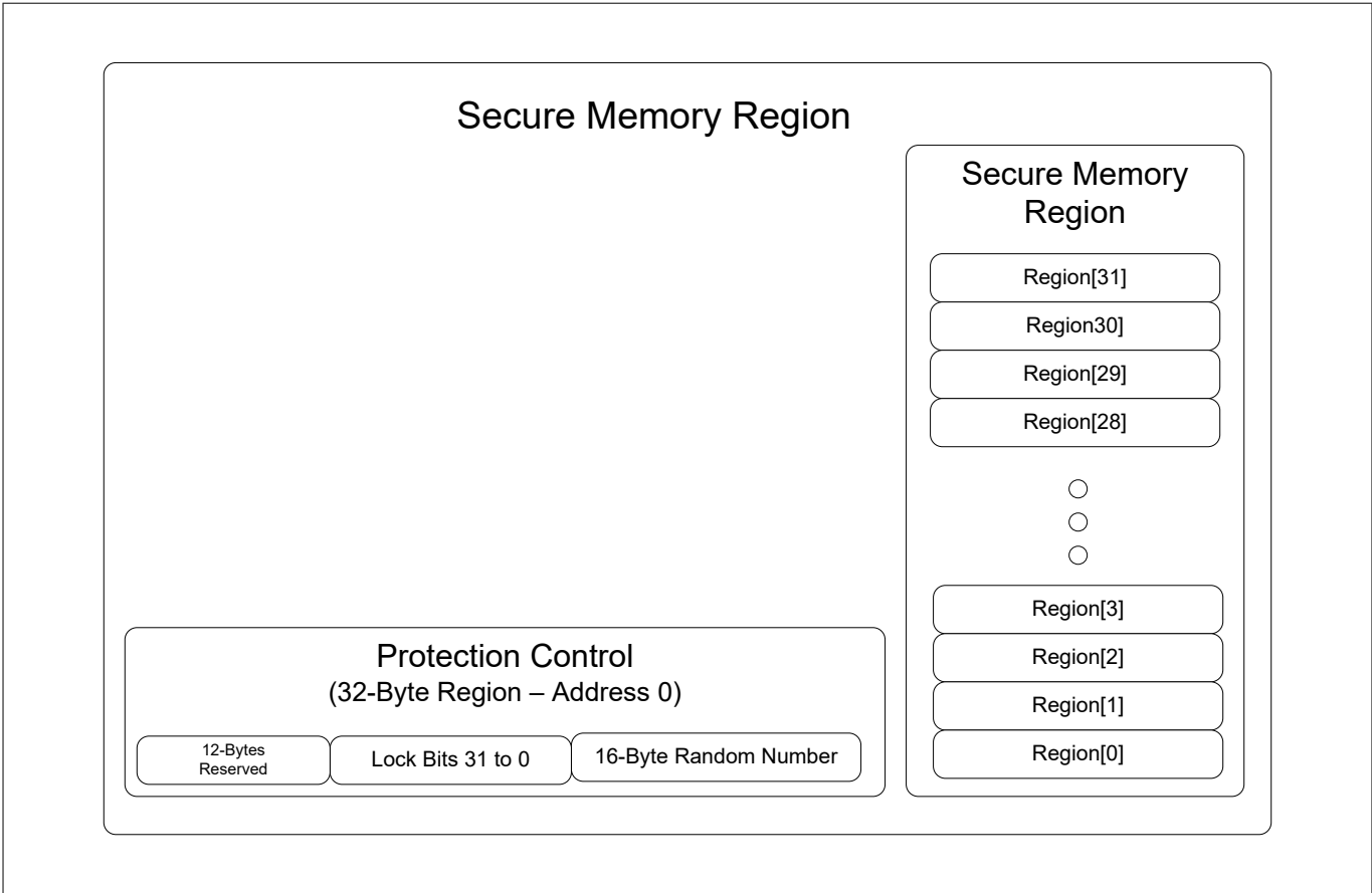
Figure 52 OTP protection (nonvolatile)
