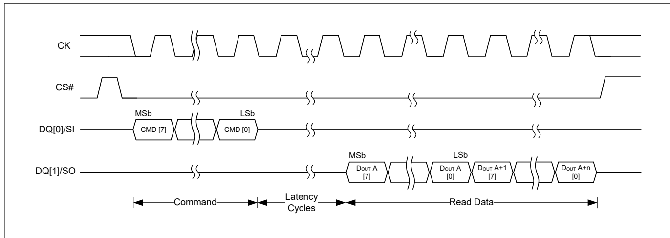
Figure 12 SPI read transaction with command input (output latency) 2), 3)
