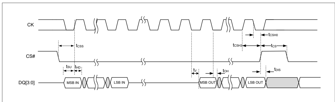
Figure 82 Quad and QPI SDR input and output timing
