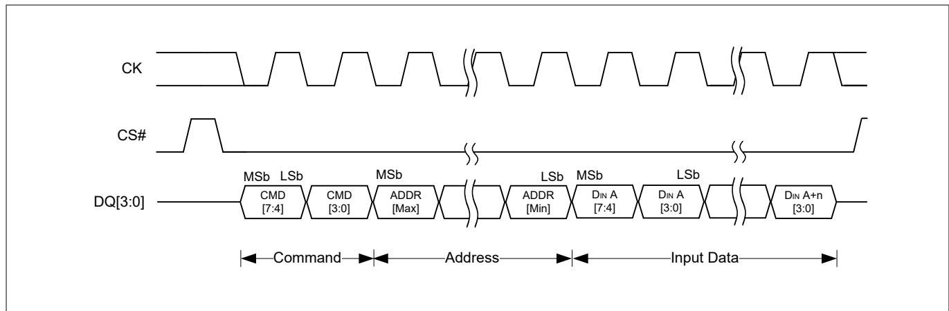
Figure 30 QPI SDR program transaction with command, address, and data input
