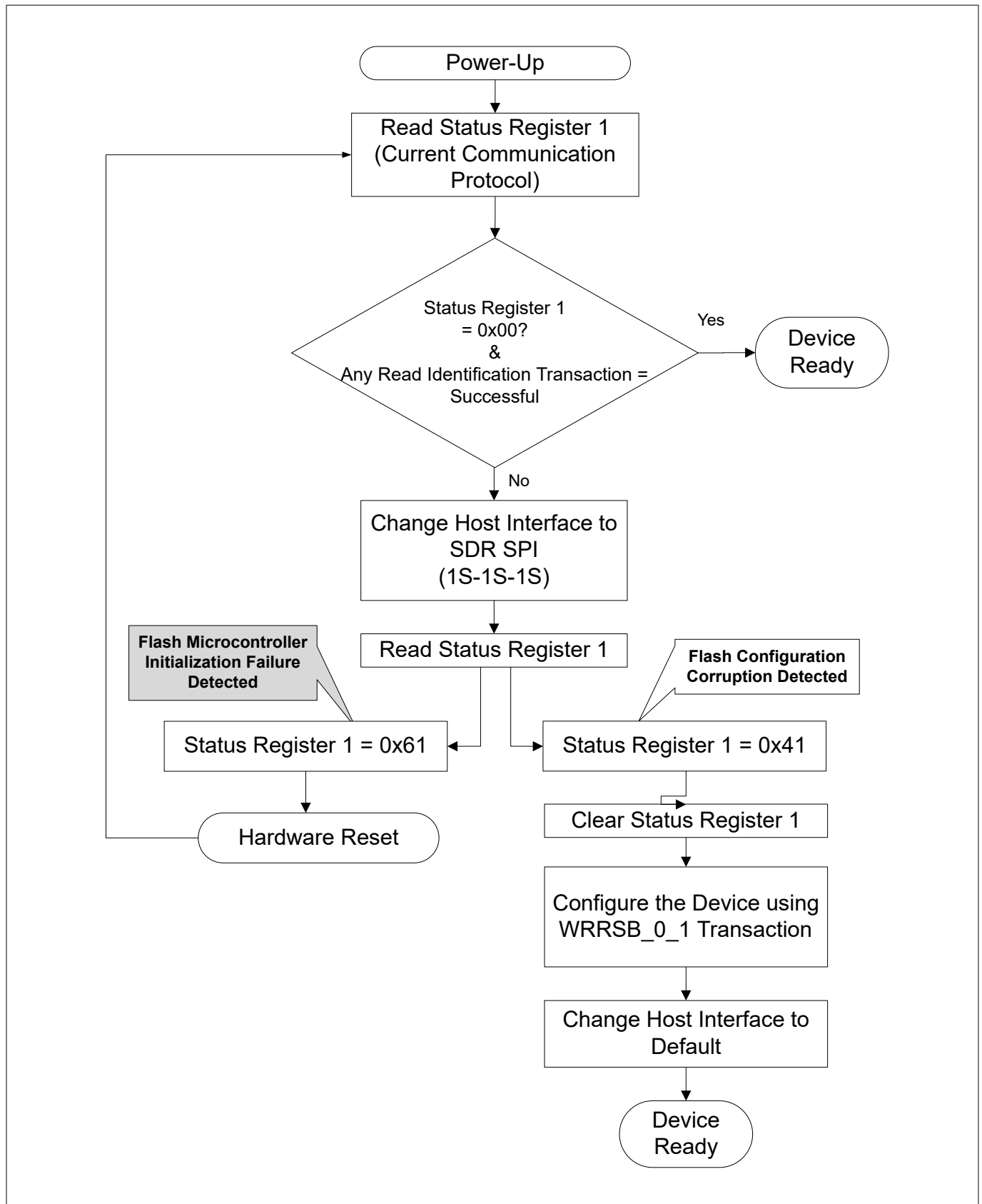
Figure 53 Host polling sequence for microcontroller initialization failure detection
