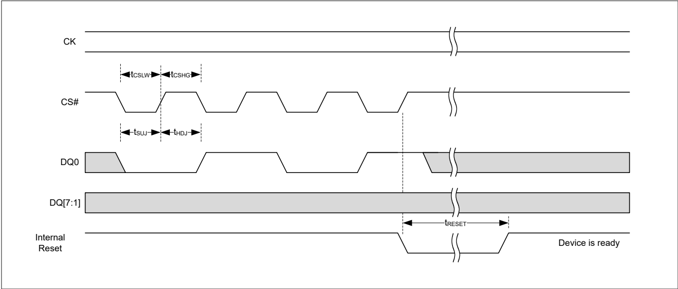
Figure 63 JEDEC serial flash reset signaling protocol
