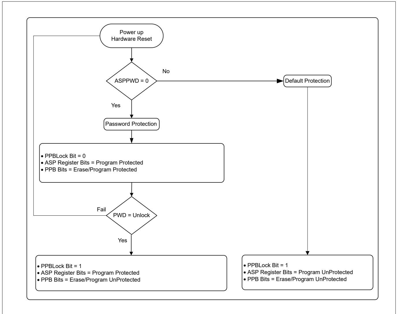
Figure 50 Password protection scheme flowchart
