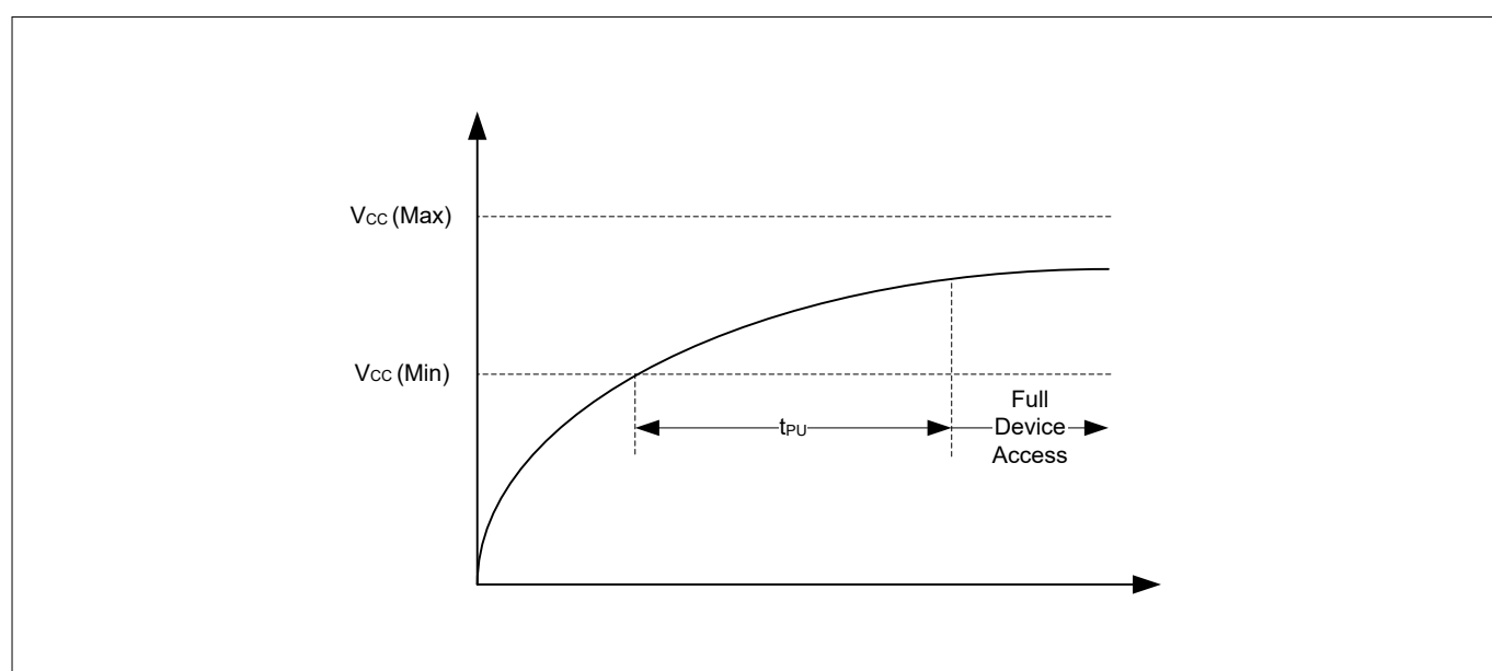
Figure 66 Power up
