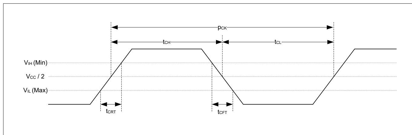
Figure 78 Clock timing
