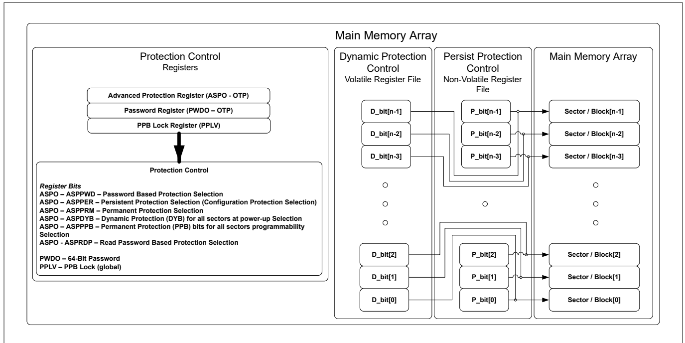
Figure 45 Advanced sector protection (Nonvolatile)
