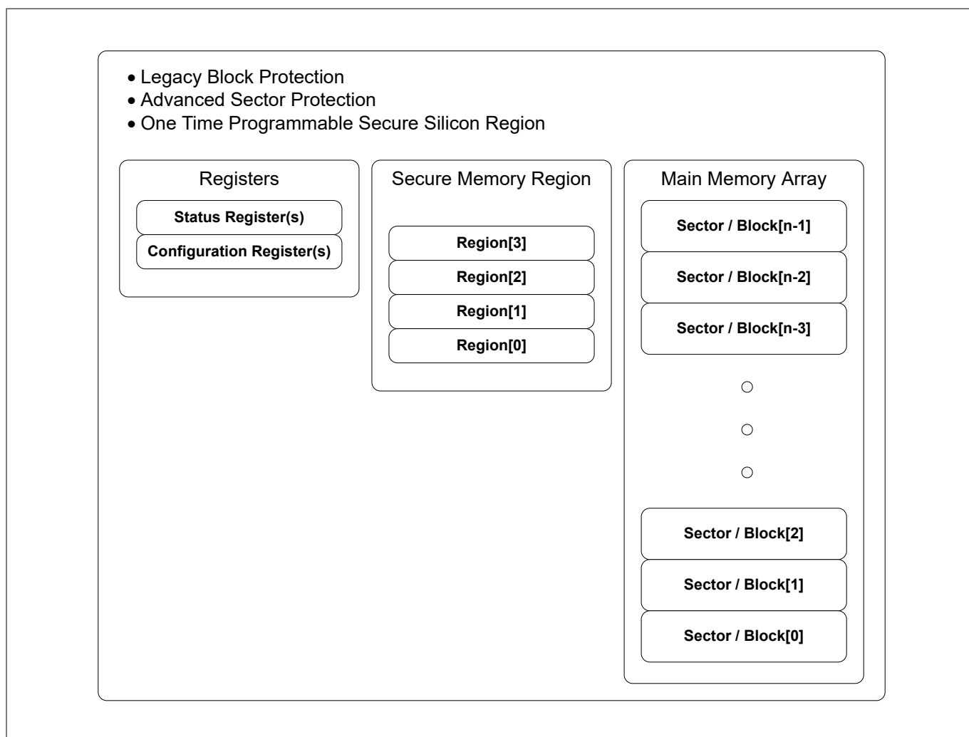
Figure 43 Data protection and security (write/program/erase) schemes
