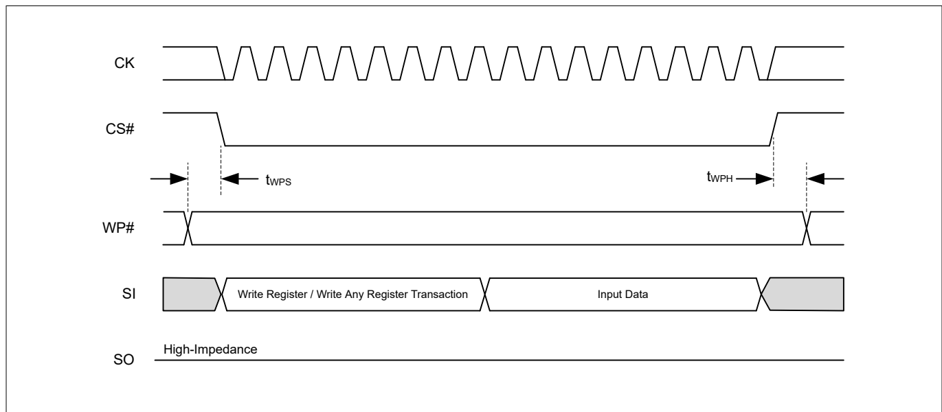
Figure 81 WP# input timing
