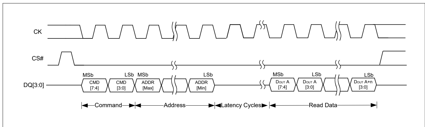
Figure 31 QPI SDR read transaction with command and address input (output latency)
