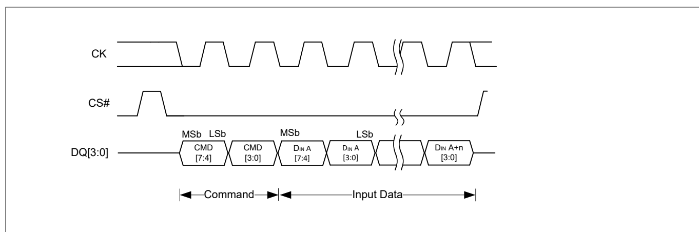
Figure 29 QPI SDR transaction with command and data input
