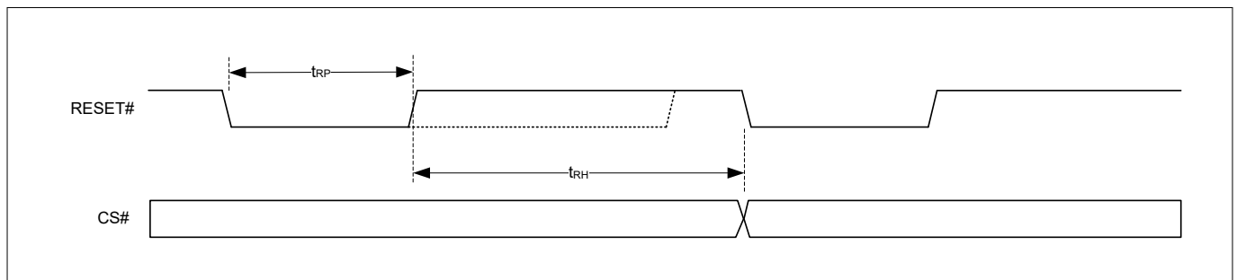
Figure 58 Hardware reset using RESET# input (back to back hardware reset)
