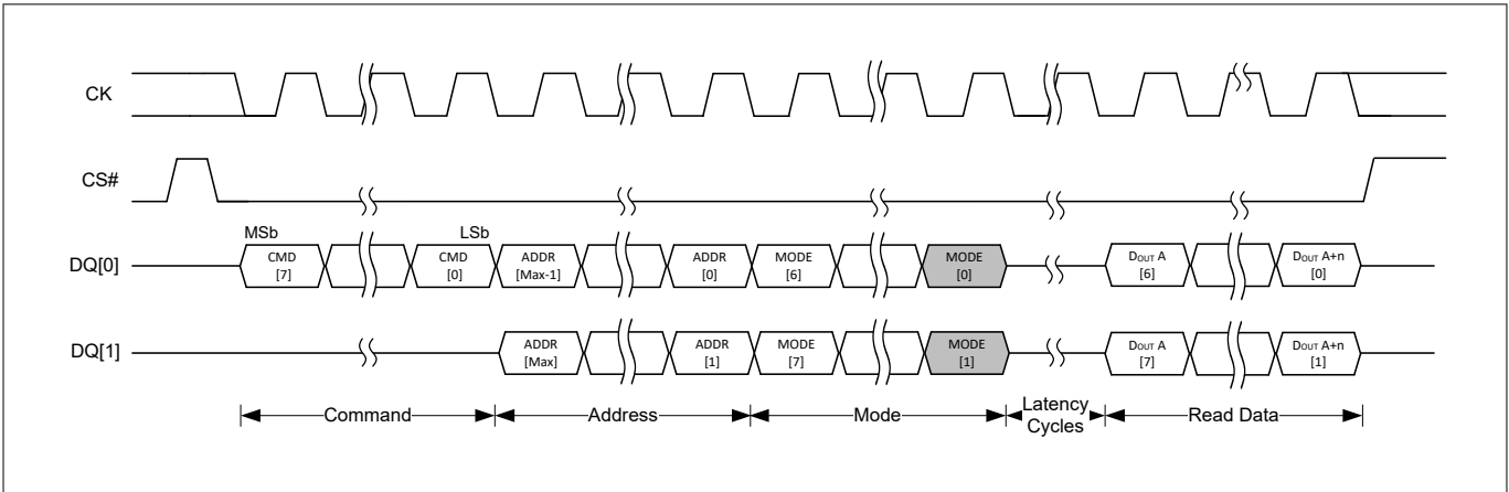
Figure 16 DIO read transaction with command, address, and mode input (output latency)
