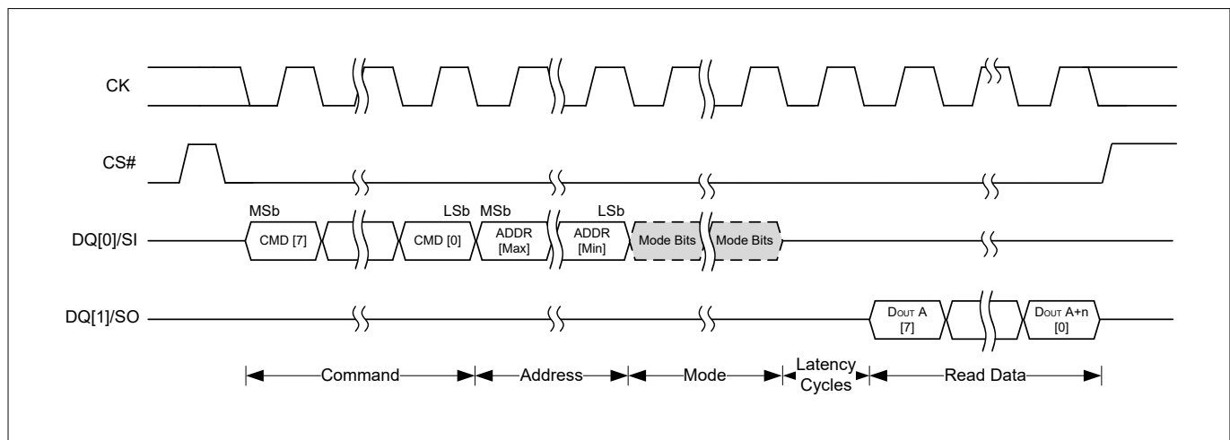
Figure 13 SPI read transaction with command and address input (output latency) 4)
