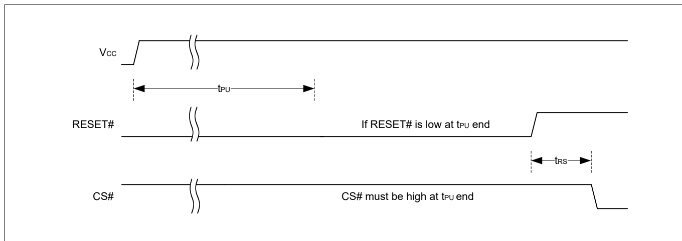
Figure 61 Reset LOW at the end of POR
