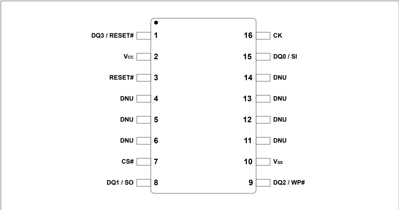
Figure 2 16-lead SOIC package (SO316), top view
