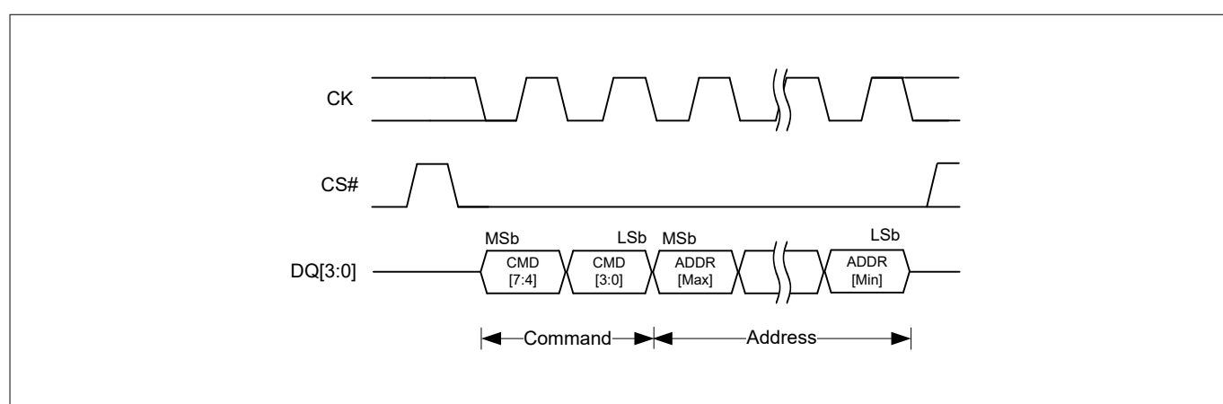
Figure 26 QPI SDR transaction with command and address input
