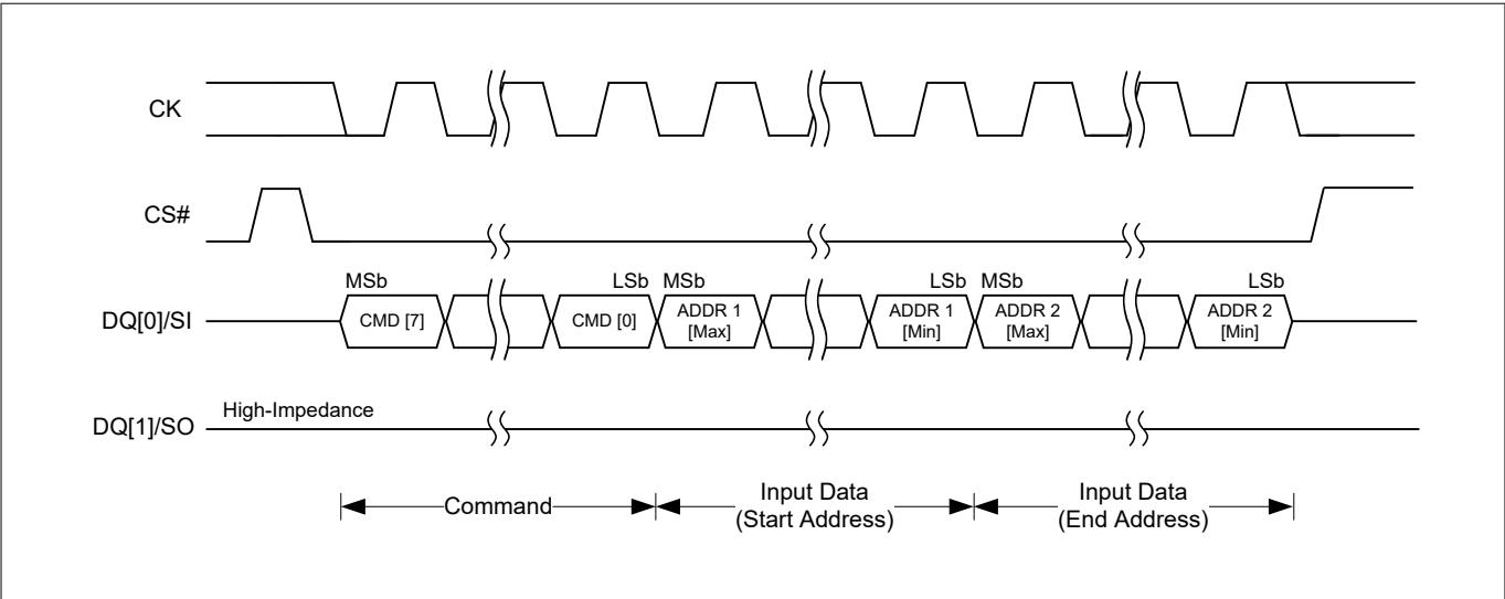
Figure 9 SPI transaction with command and two input addresses
