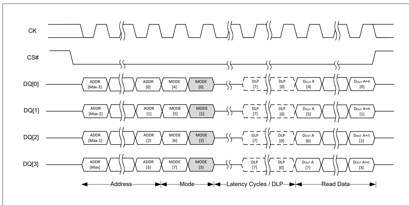
Figure 20 QIO SDR continuous read transaction with address and mode input (output latency) 5)
