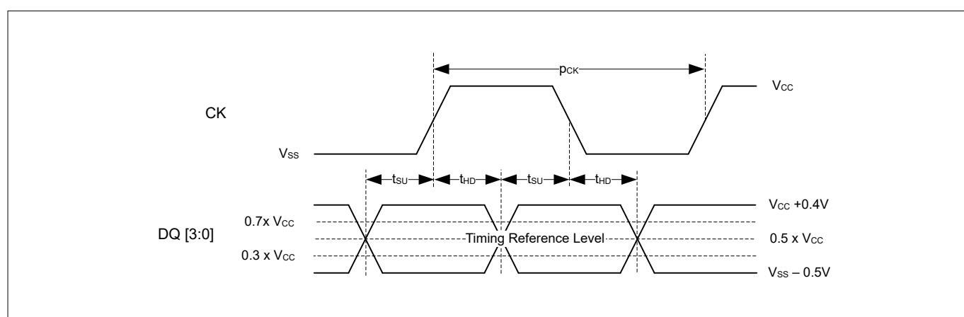
Figure 76 DDR input timing reference level
