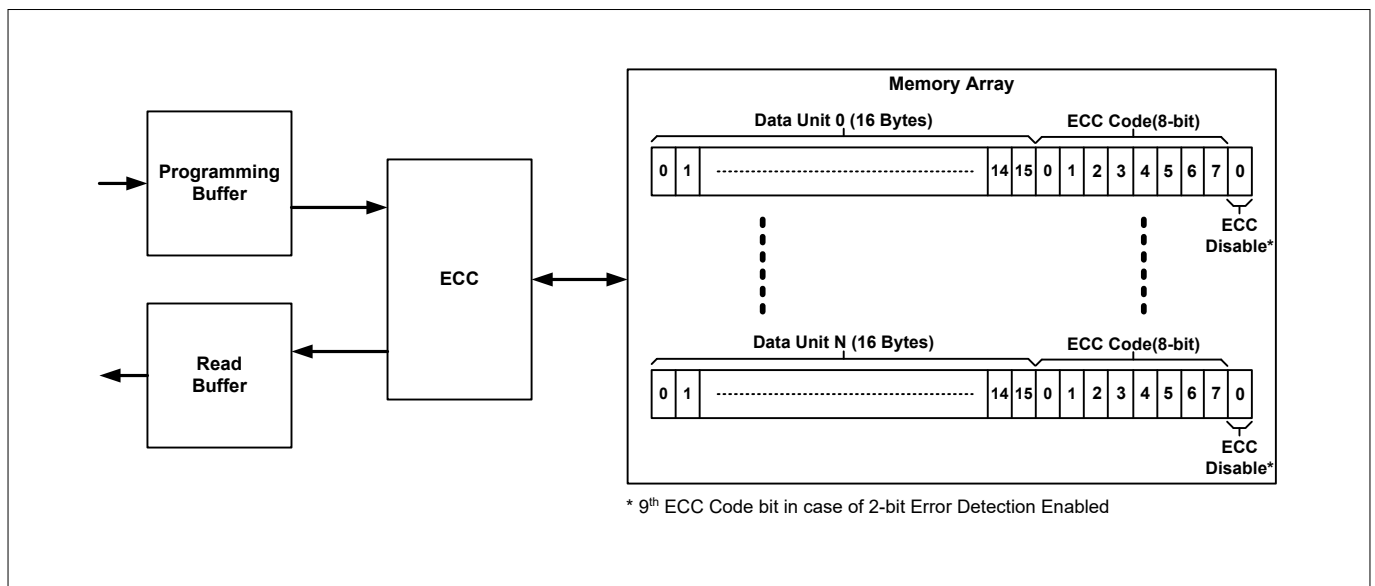
Figure 40 16-byte ECC data unit example
