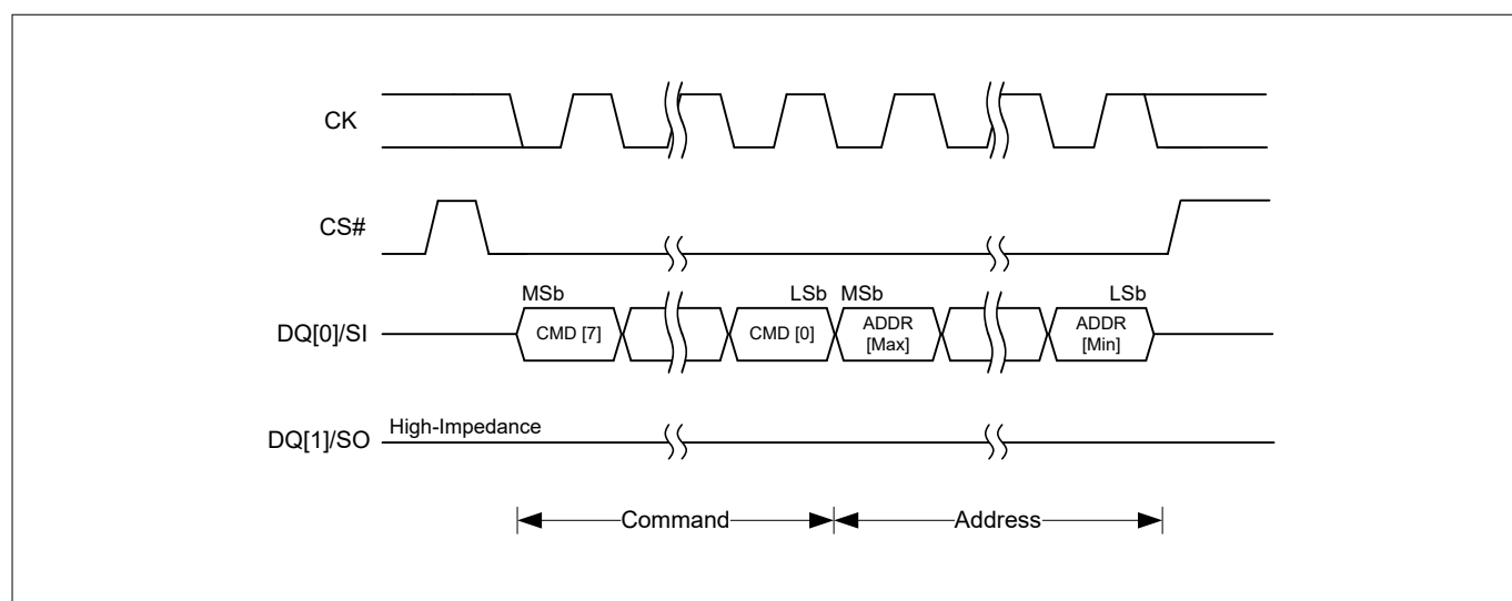
Figure 8 SPI transaction with command and address input
