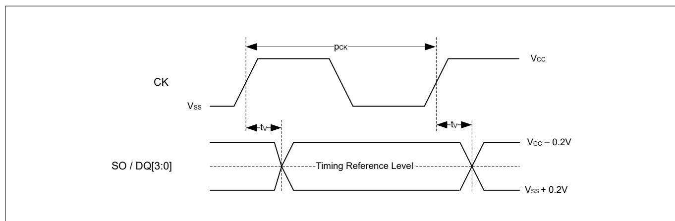
Figure 75 SDR output timing reference level
