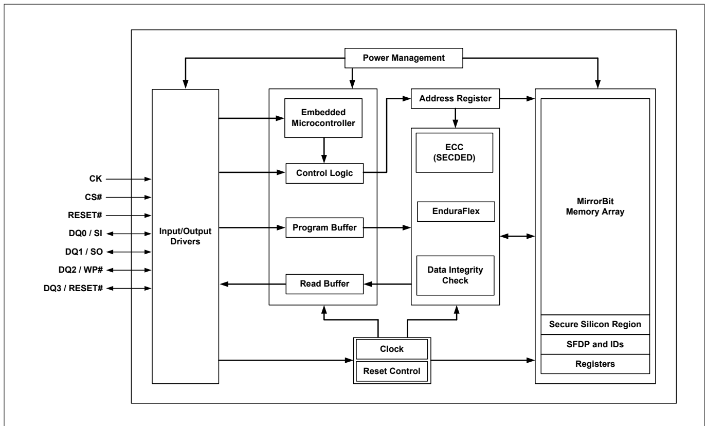
Figure 4 Logic block diagram
