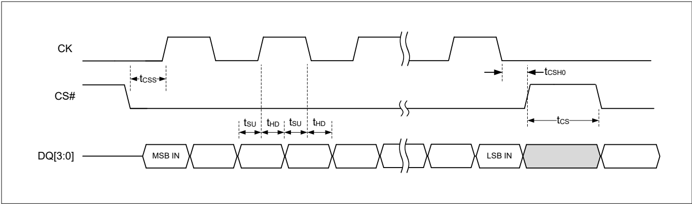
Figure 83 Quad and QPI DDR input timing
