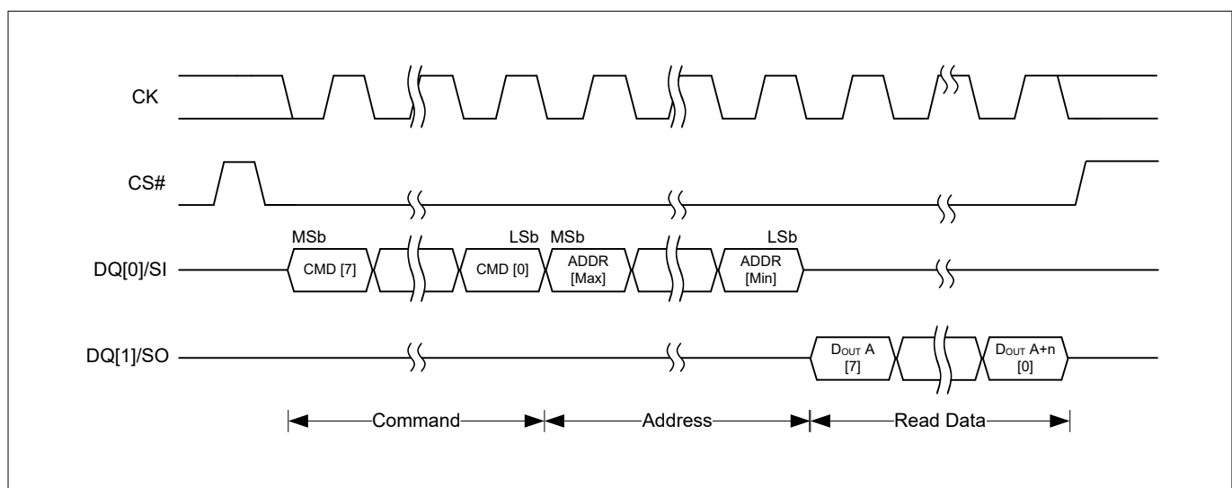
Figure 14 SPI read transaction with command and address input (no output latency)
