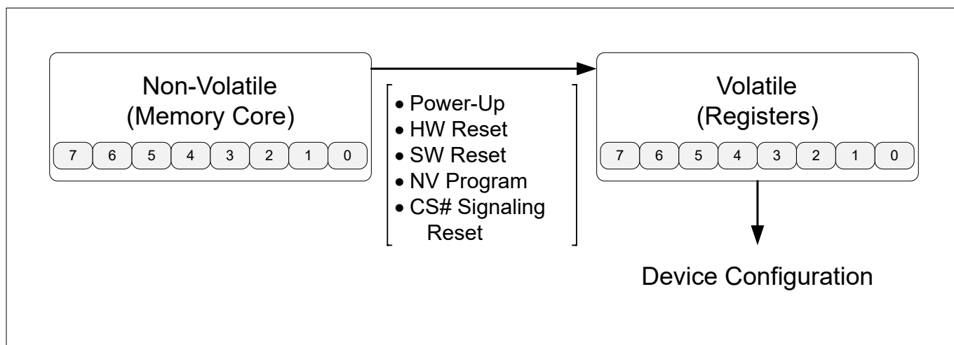
Figure 69 Data movement within register components
