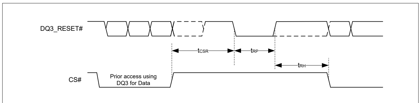
Figure 60 Hardware reset when quad or QPI mode and DQ3_RESET# are enabled
