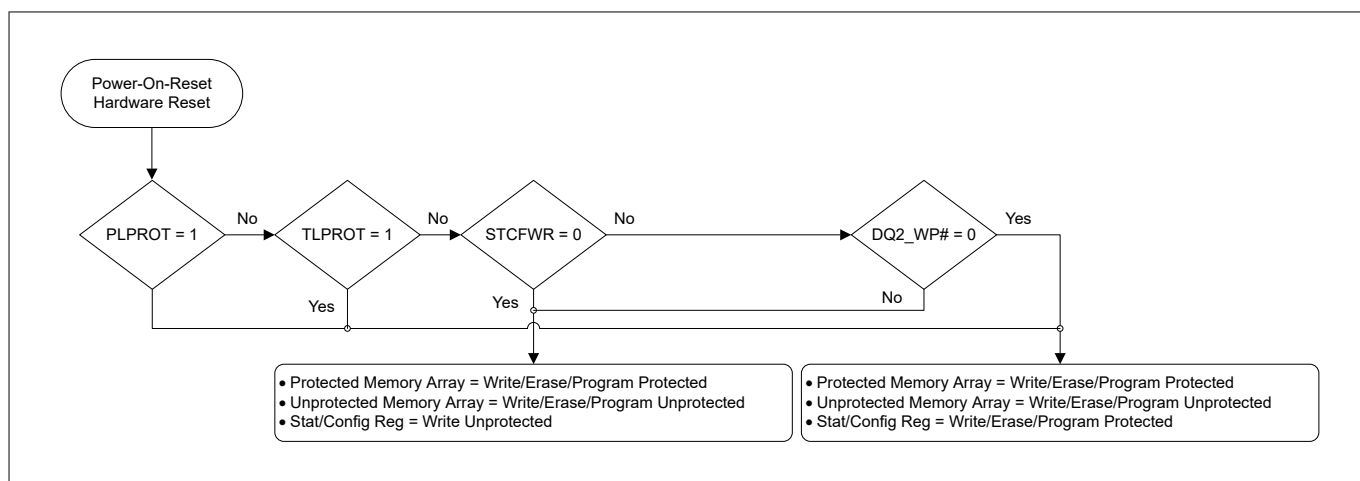
Figure 44 Legacy block protection flowchart
