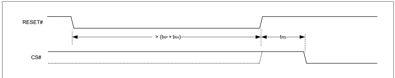
Figure 57 Hardware reset using RESET# input (reset pulse > ( t_{RP} + t_{RH} ))
