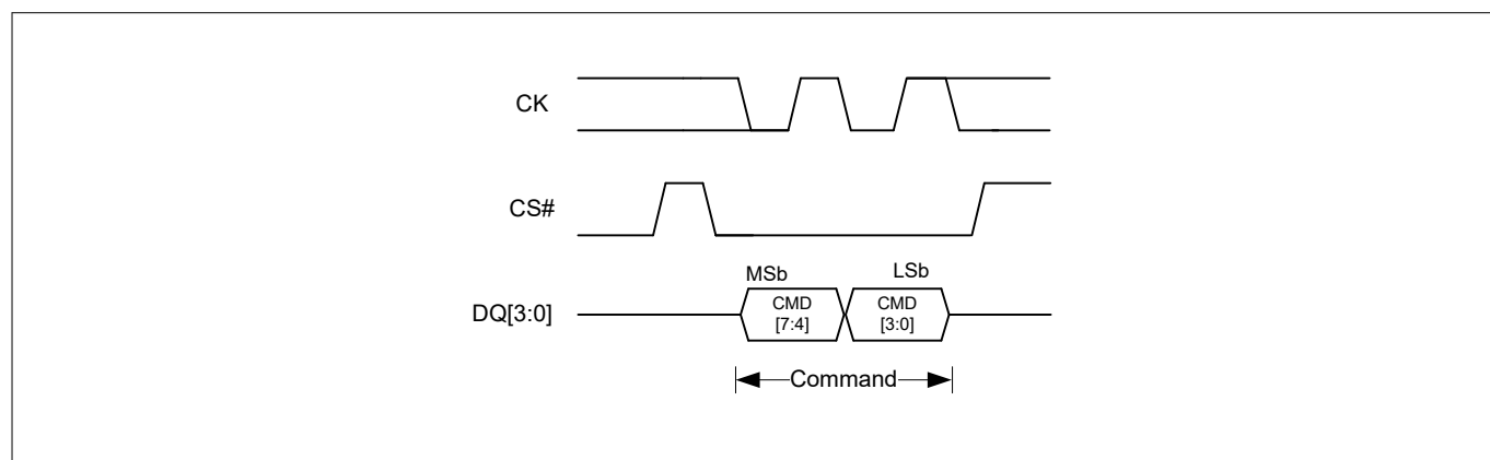
Figure 24 QPI SDR transaction with command input
