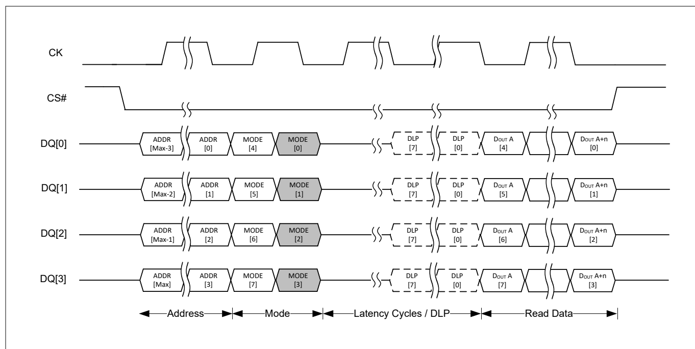
Figure 22 QIO DDR continuous read transaction with address and mode input (output latency)
