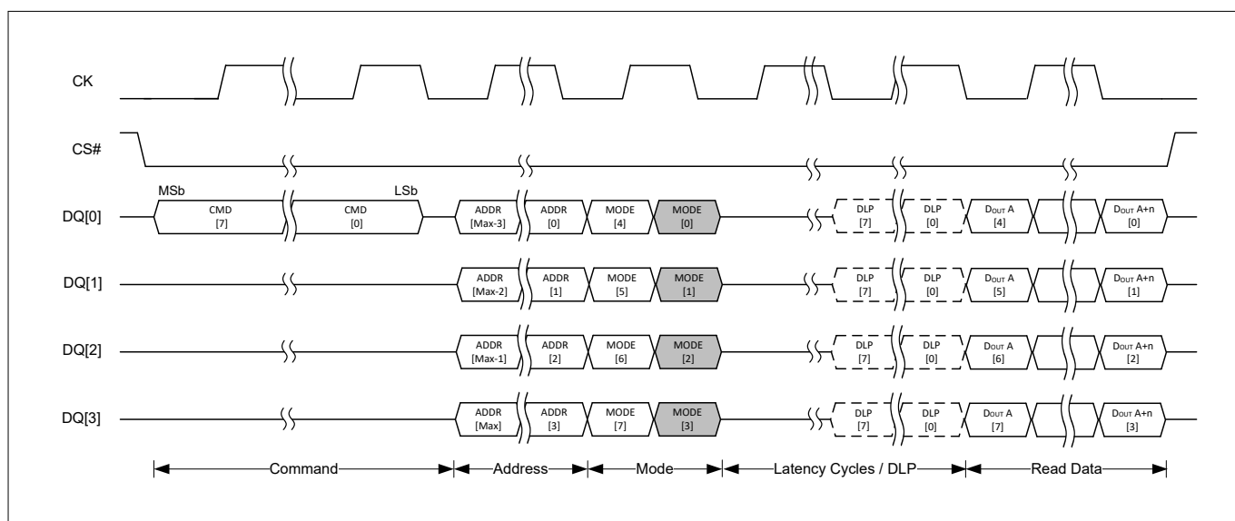
Figure 21 QIO DDR read transaction with command, address, and mode input (output latency)
