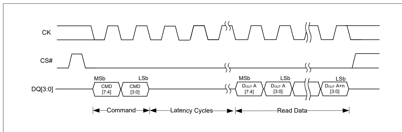
Figure 27 QPI SDR read transaction with command input (output latency)
