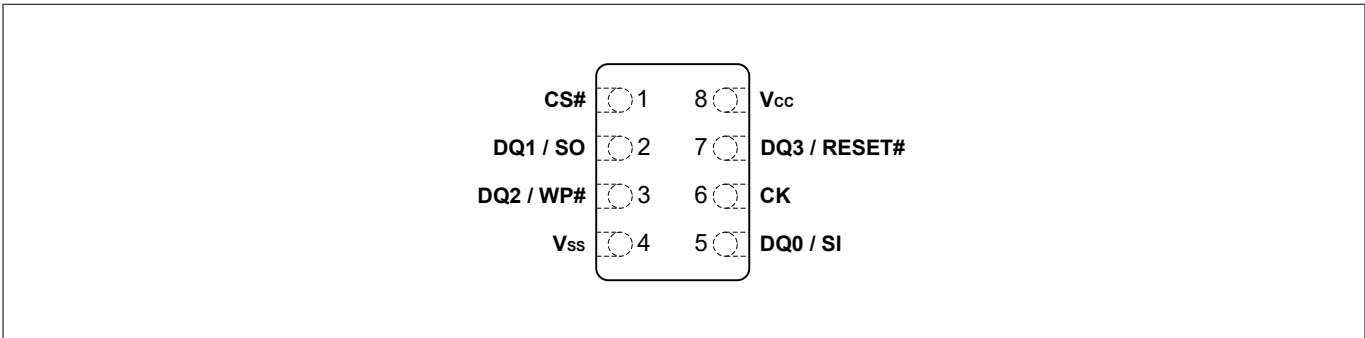
Figure 3 8-connector package (WSON 6 × 8), top view
