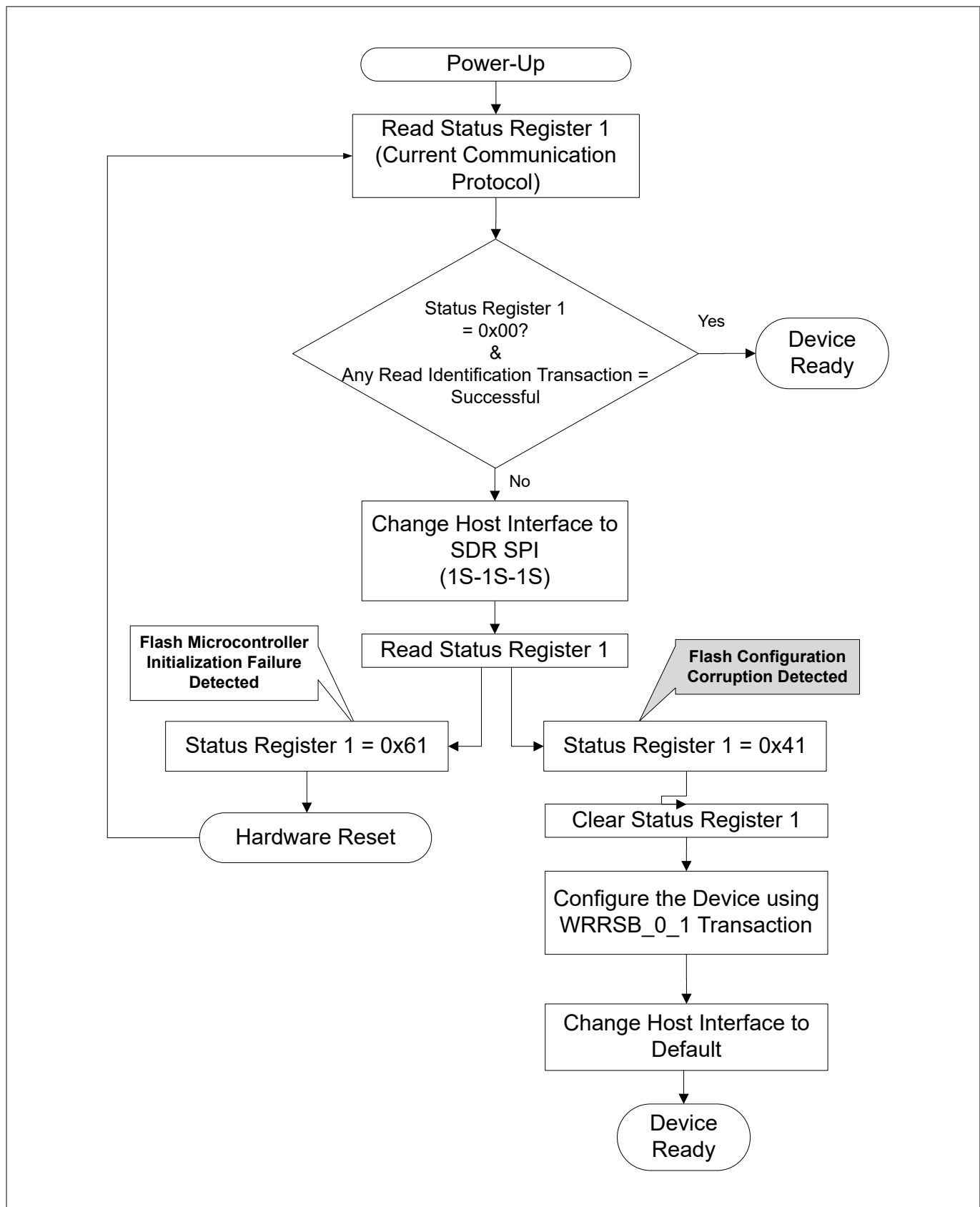
Figure 54 Host polling sequence for configuration corruption detection
