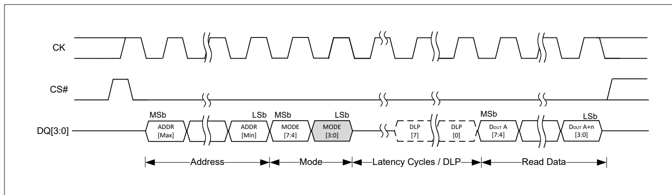
Figure 33 QPI SDR continuous read transaction with address and mode input (output latency) 6)
