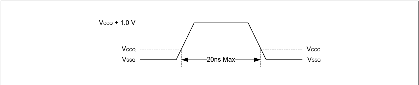
Figure 71 Maximum positive overshoot waveform
