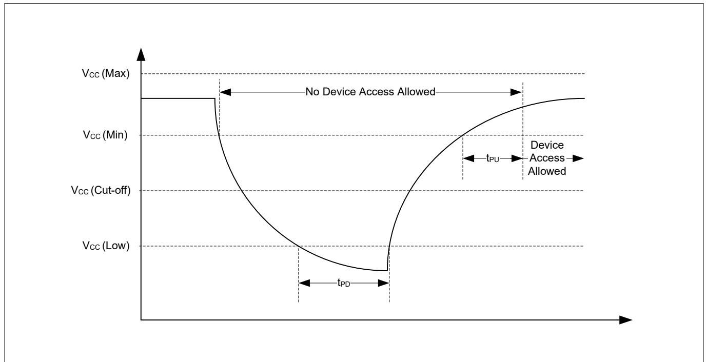
Figure 67 Power down and voltage drop
