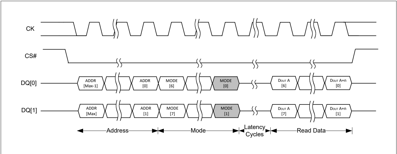
Figure 17 DIO continuous read transaction with address and mode input (output latency)
