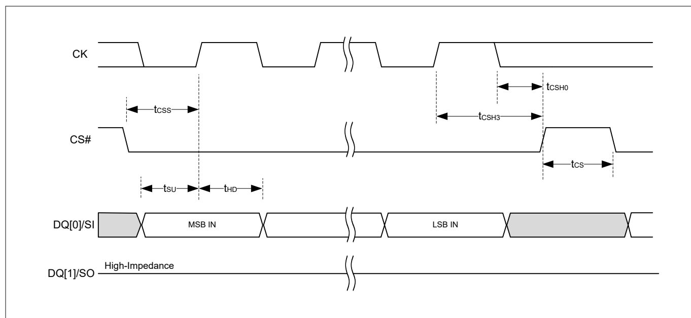
Figure 79 SPI input timing
