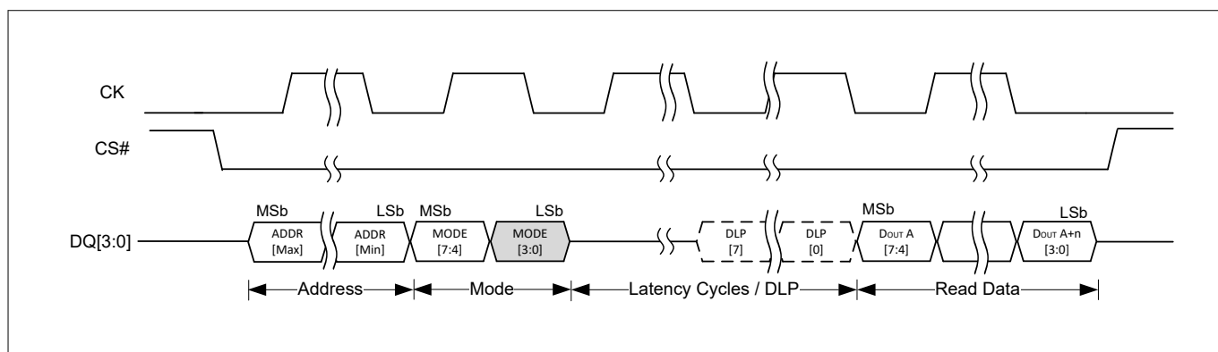
Figure 35 QPI DDR continuous read transaction with address and mode input (output latency) 6)
