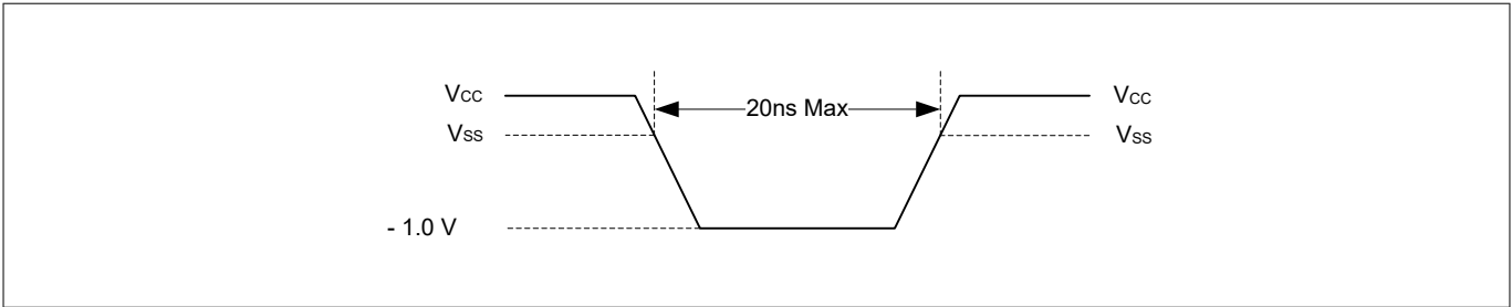
Figure 70 Maximum negative overshoot waveform
