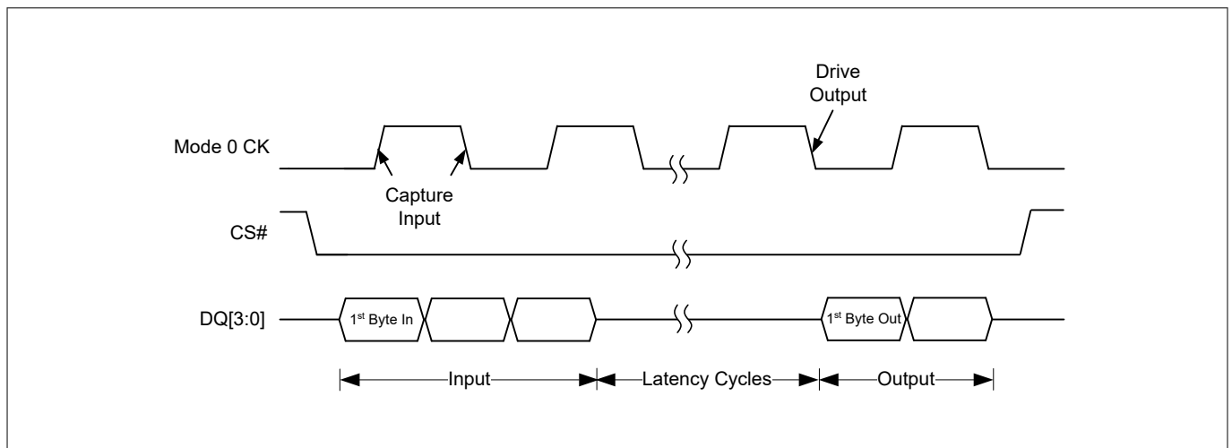
Figure 6 SPI DDR mode support
