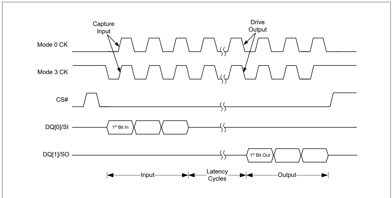
Figure 5 SPI SDR mode support
