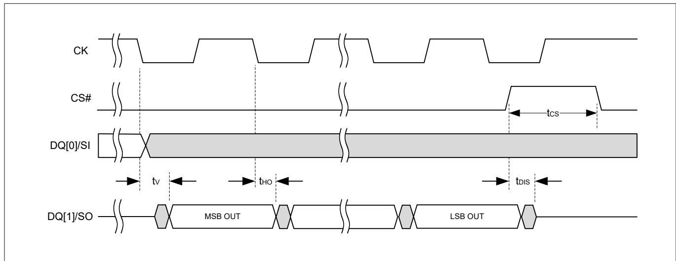
Figure 80 SPI output timing
