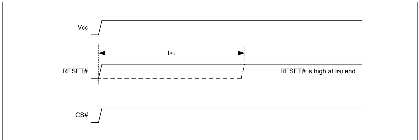
Figure 64 Enter DPD mode upon power-up or reset
