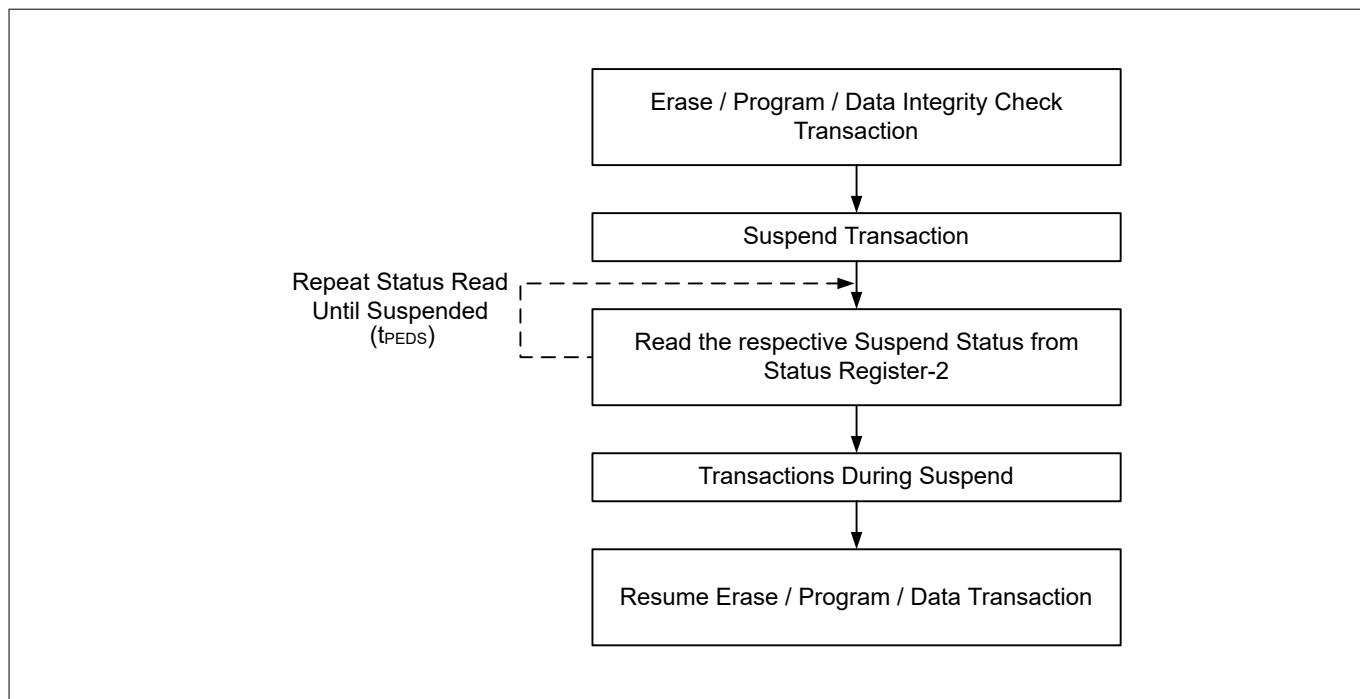
Figure 55 Suspend and resume sequence
