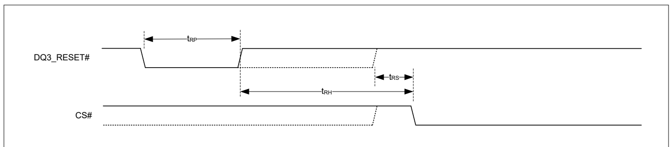
Figure 59 Hardware reset when quad or QPI mode is disabled and DQ3_RESET# is enabled
