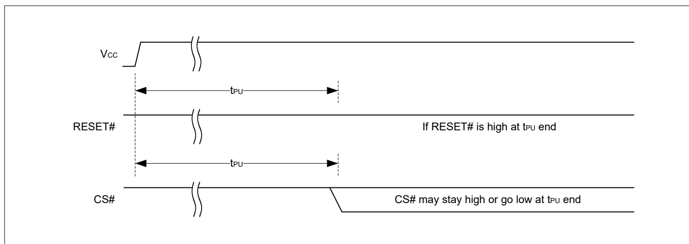
Figure 62 Reset HIGH at the end of POR
