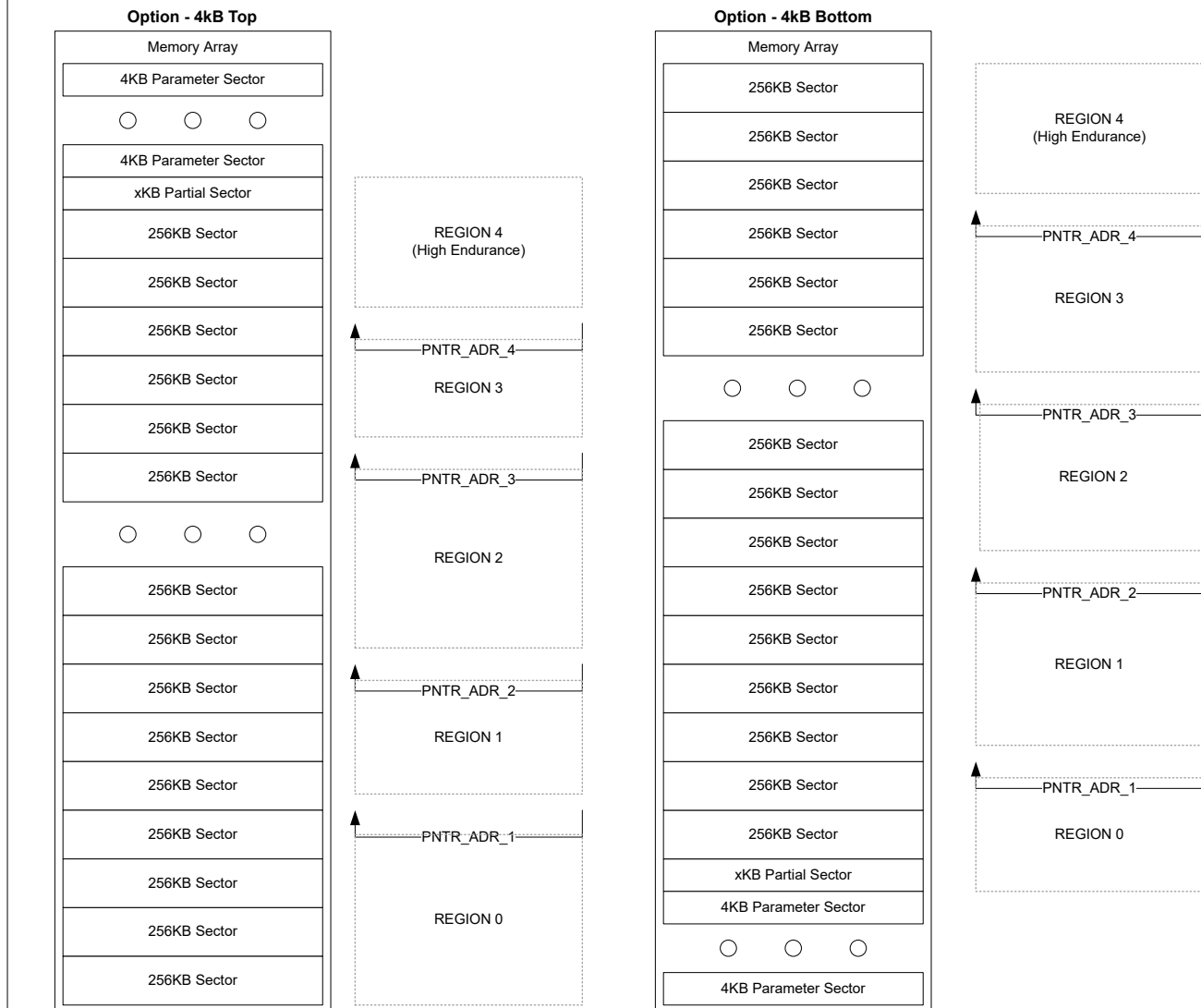
Figure 41 Infineon Endurance Flex architecture overview
