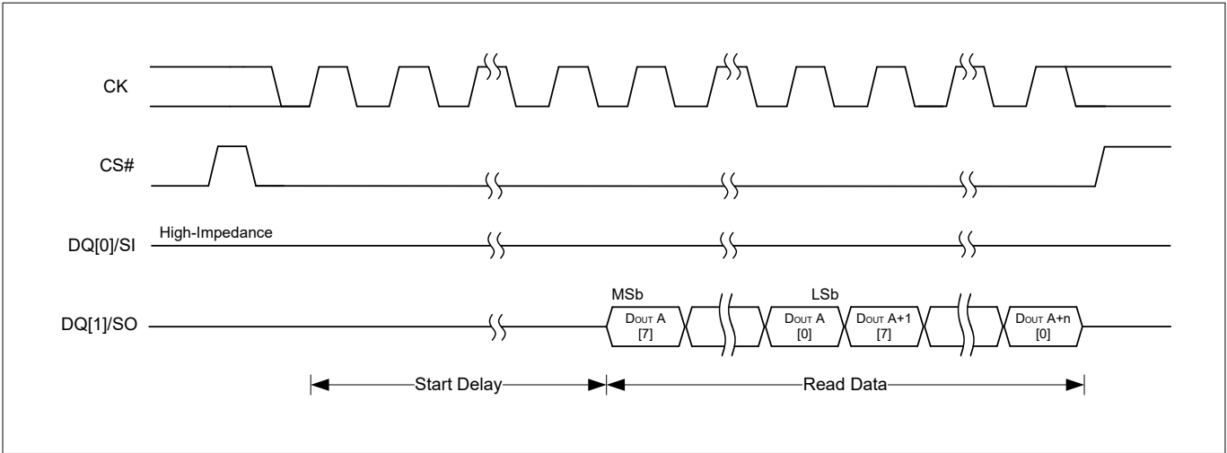
Figure 15 SPI transaction with output data sequence (AutoBoot)
