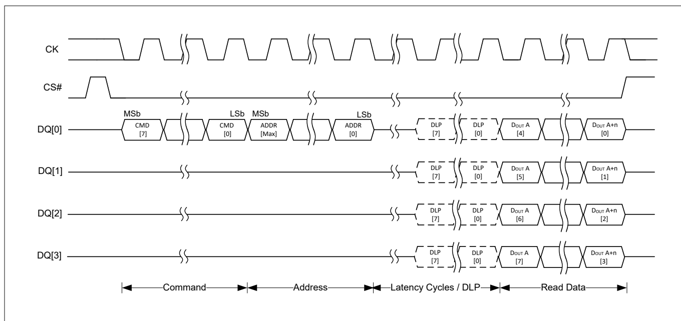
Figure 18 QOR SDR read transaction with command, address, and mode input (output latency)
