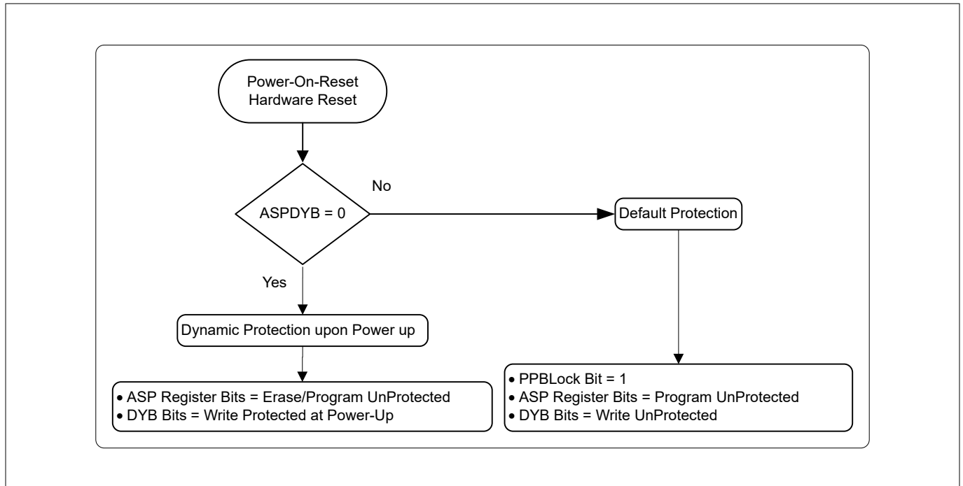
Figure 48 Dynamic sector protection scheme flowchart
