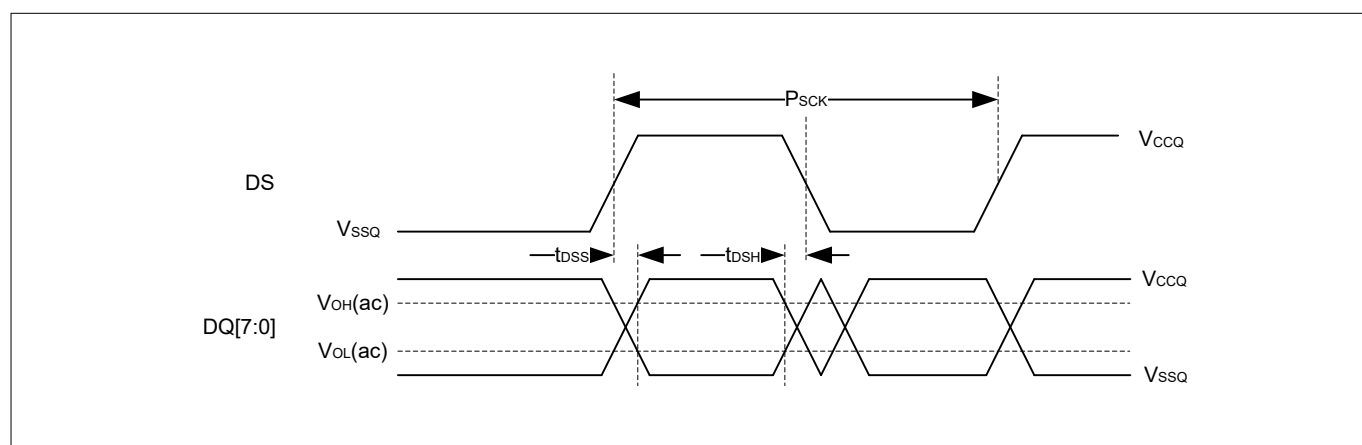
Figure 77 DDR output timing reference level
