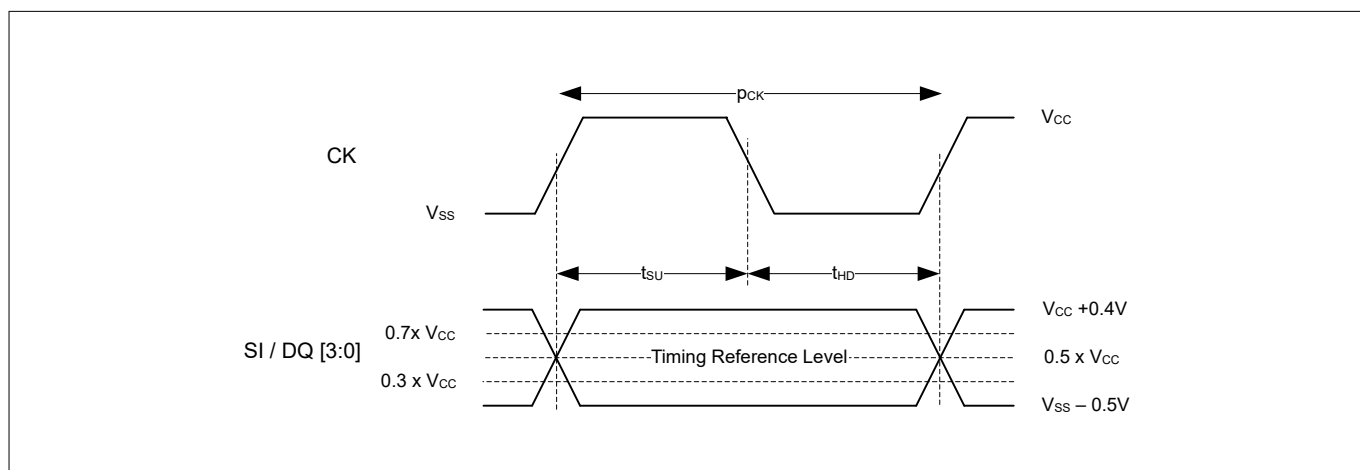
Figure 74 SDR input timing reference levels
