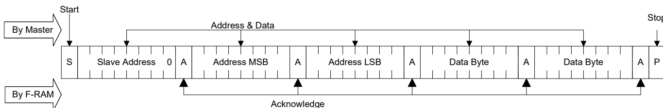
Figure 9. Multi-Byte Write
