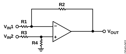
Figure 2. Difference Amplifier
