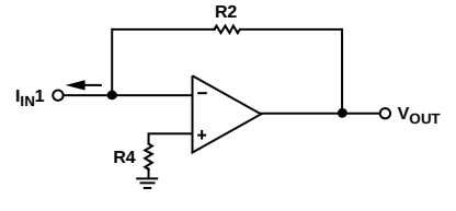
Figure 3. Current-to-Voltage Converter
