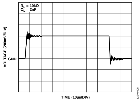
Figure 5. Capacitive Load Drive Without Resistor
