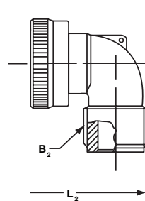
CB6T ENDBELL
