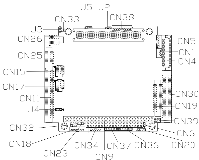
Figure 2.1 Connectors (component side)
