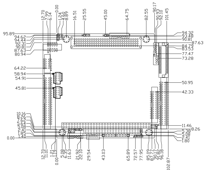
Figure C.1 PCM-4153 Mech drawing (comp side)
