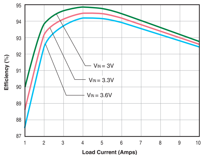
LSM-2.5/10-D3 Efficiency vs. Line Voltage and Load Current
