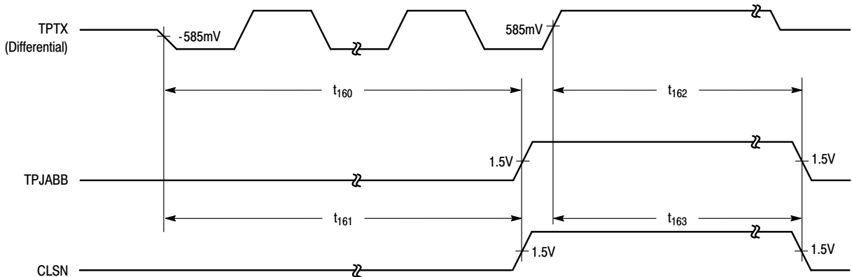
Figure 28. TPJABB Switching
