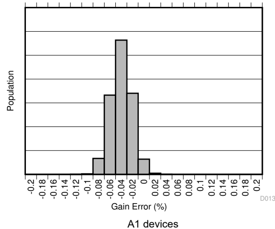
Figure 6-5. Gain Error Production Distribution
