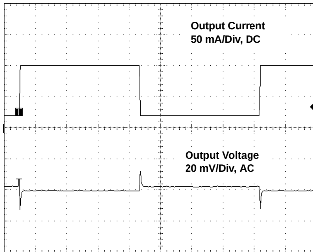
LDO LOAD TRANSIENT RESPONSE
