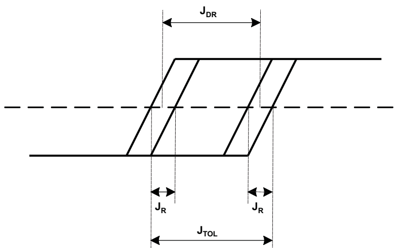
Figure 4-4. Input Jitter
