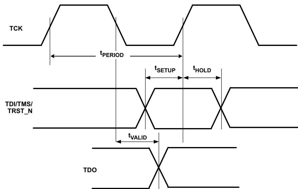
Figure 4-14. JTAG Timing
