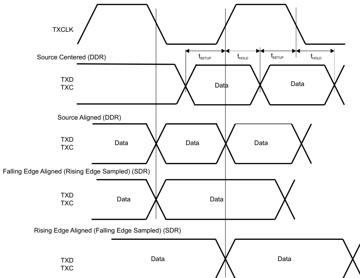
Figure 2-18. Transmit Interface Timing
