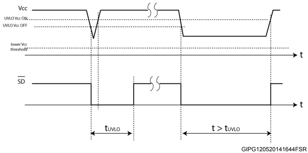
Figure 5. UVLO timing (without contribution of the RC network on \overline{\text{SD}} )
